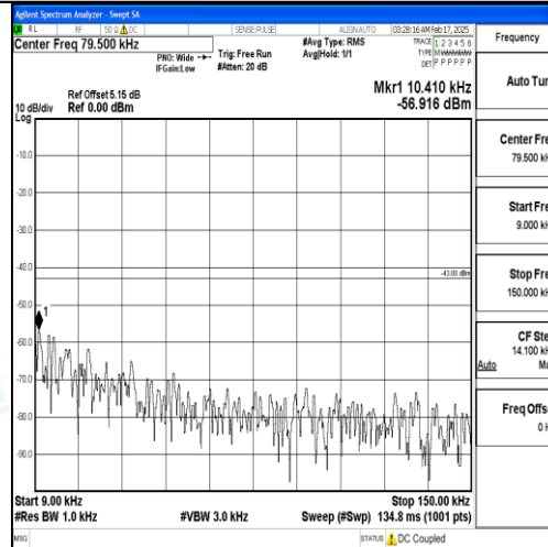
Band25_5MHz_QPSK_26365_1RB#0_0.009~0.15_0.009~0.15
