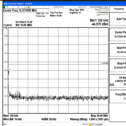
Band25_5MHz_QPSK_26365_1RB#0_0.15~30_0.15~30
