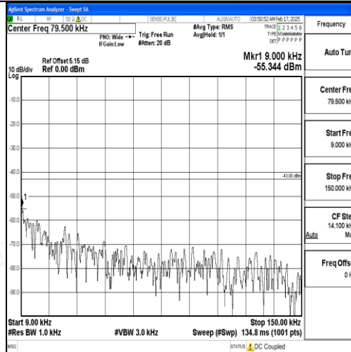
Band25_10MHz_16QAM_26640_1RB#0_0.009~0.15_0.009~0.15
