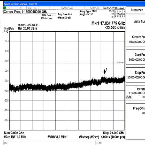
Band25_5MHz_16QAM_26065_1RB#0_3000~20000_3000~20000
