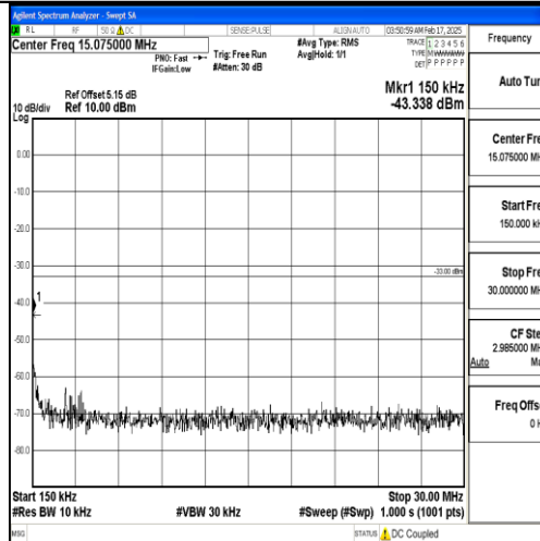
Band25_10MHz_16QAM_26640_1RB#0_0.15~30_0.15~30
