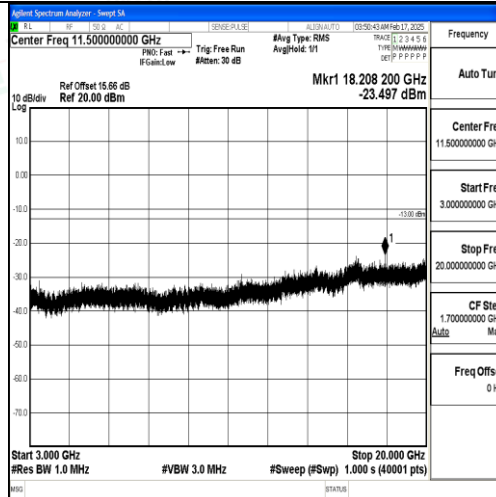
Band25_10MHz_QPSK_26640_1RB#0_3000~20000_3000~20000
