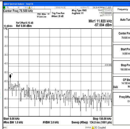
Band25_1.4MHz_16QAM_26365_1RB#0_0.009~0.15_0.009~0.15
