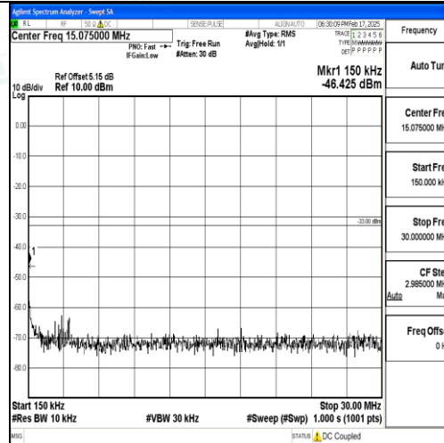
Band25_3MHz_16QAM_26055_1RB#0_0.15~30_0.15~30
