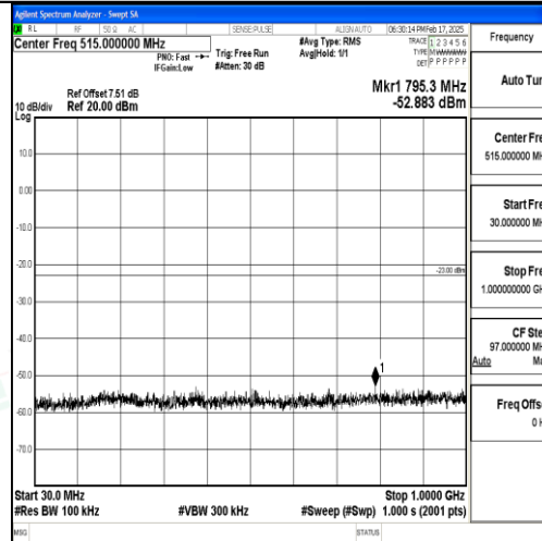
Band25_3MHz_16QAM_26055_1RB#0_30~1000_30~1000
