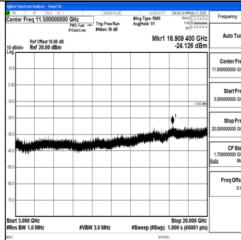
Band25_1.4MHz_QPSK_26365_1RB#0_3000~20000_3000~20000
