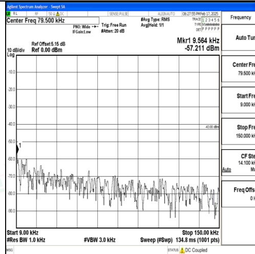
Band25_1.4MHz_16QAM_26683_1RB#0_0.009~0.15_0.009~0.15
