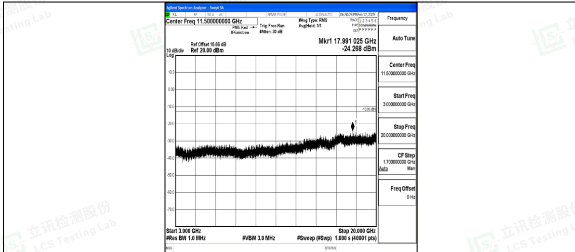
Band25_3MHz_16QAM_26055_1RB#0_3000~20000_3000~20000
