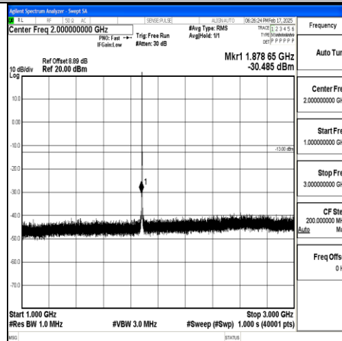
Band25_1.4MHz_QPSK_26365_1RB#0_1000~3000
