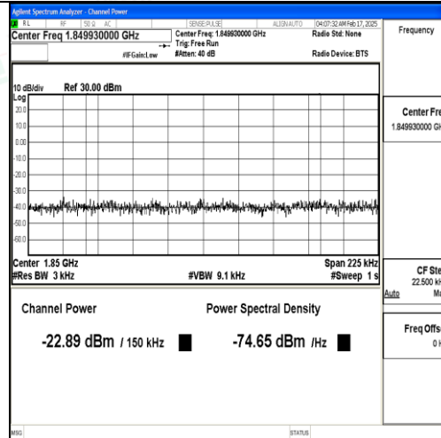
Band25_15MHz_QPSK_26115_75RB#0_Final1
