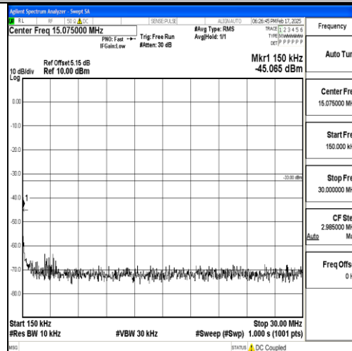
Band25_1.4MHz_16QAM_26365_1RB#0_0.15~30_0.15~30
