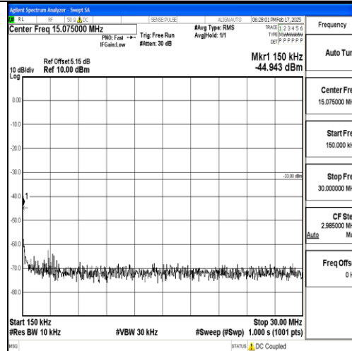
Band25_1.4MHz_16QAM_26683_1RB#0_0.15~30_0.15~30
