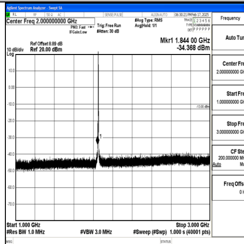
Band25_3MHz_16QAM_26055_1RB#0_1000~3000_1000~3000
