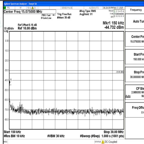
Band25_1.4MHz_QPSK_26365_1RB#0_0.15~30
