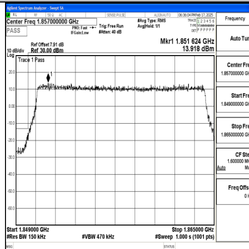
Band25_15MHz_16QAM_26115_75RB#0
