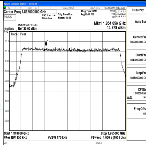
Band25_15MHz_QPSK_26115_75RB#0
