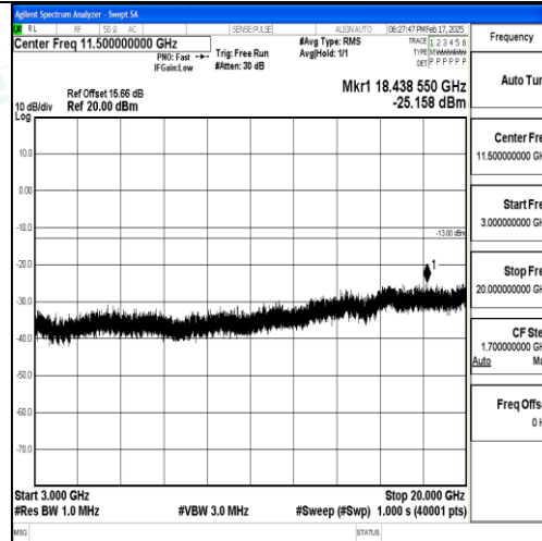
Band25_1.4MHz_QPSK_26683_1RB#0_3000~20000_3000~20000
