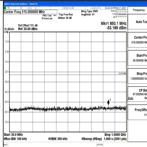
Band25_1.4MHz_QPSK_26365_1RB#0_30~1000
