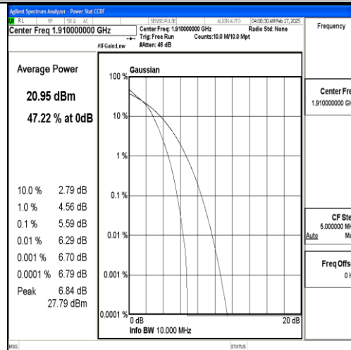
Band25-10MHz-16QAM-26640-50RB#0-PASS
