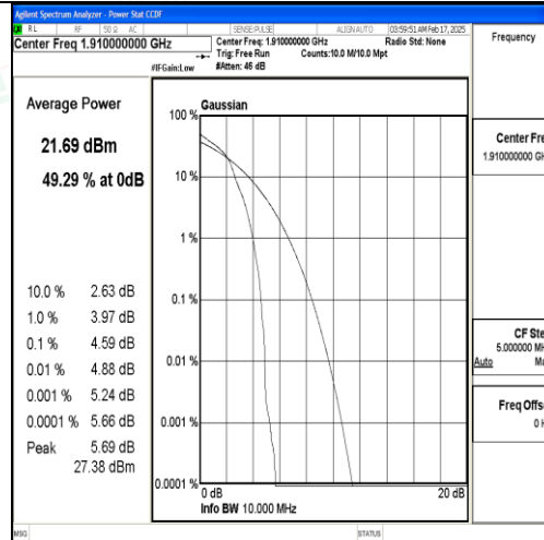
Band25-10MHz-16QAM-26640-1RB#0-PASS
