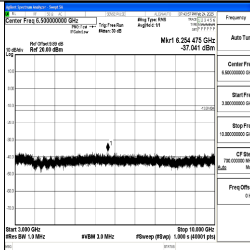
Band5_10MHz_QPSK_20450_1RB#0_3000~10000_3000~10000
