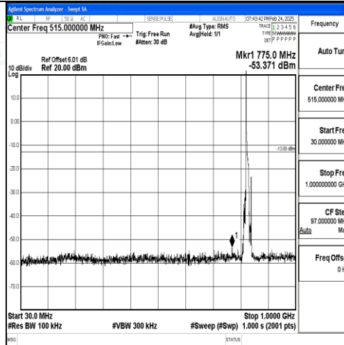
Band5_10MHz_QPSK_20450_1RB#0_30~1000_30~1000
