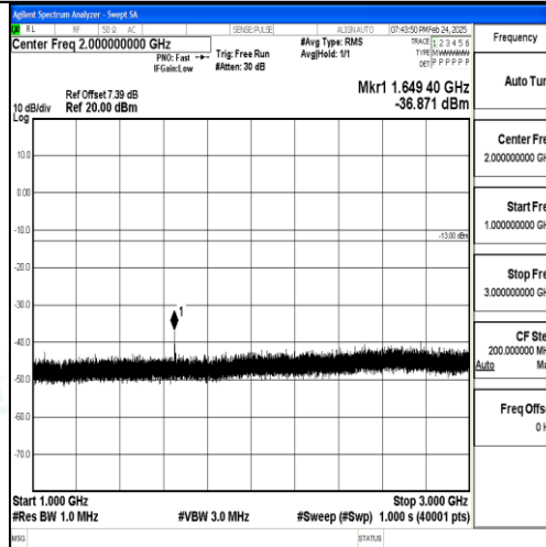
Band5_10MHz_QPSK_20450_1RB#0_1000~3000_1000~3000
