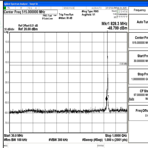
Band5_3MHz_16QAM_20525_1RB#0_30~1000_30~1000
