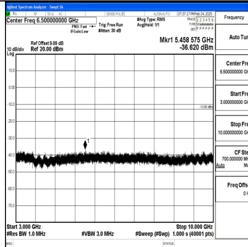
Band5_3MHz_16QAM_20525_1RB#0_3000~10000_3000~10000
