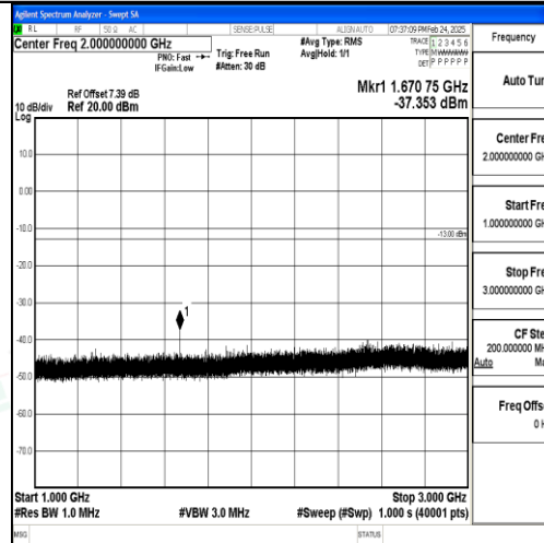
Band5_3MHz_16QAM_20525_1RB#0_1000~3000_1000~3000
