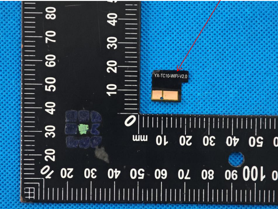
WIFI Antenna
