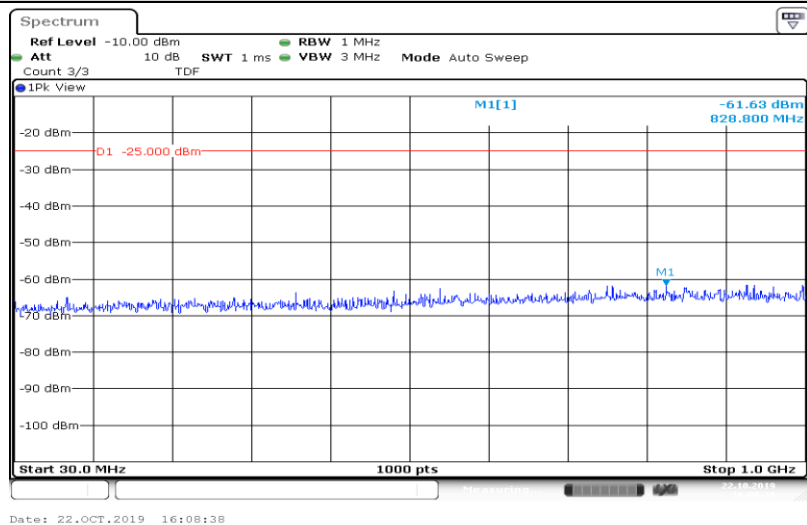
Band41-15MHz-QPSK-40315-75RB#0-Range4:1000~3000MHz
