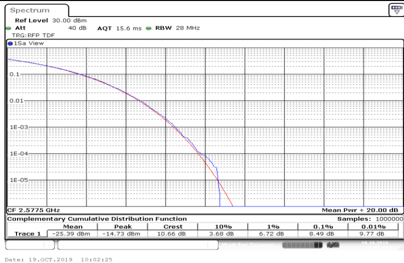
Band38-15MHz-16QAM-38000-75RB#0
