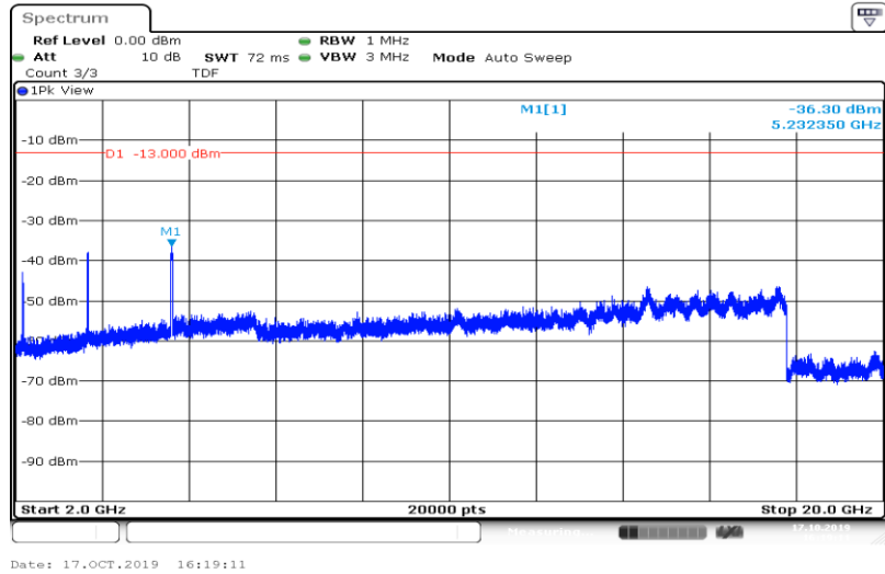
Band4-20MHz-16QAM-20050-100RB#0-Range1:0.009~0.15MHz
