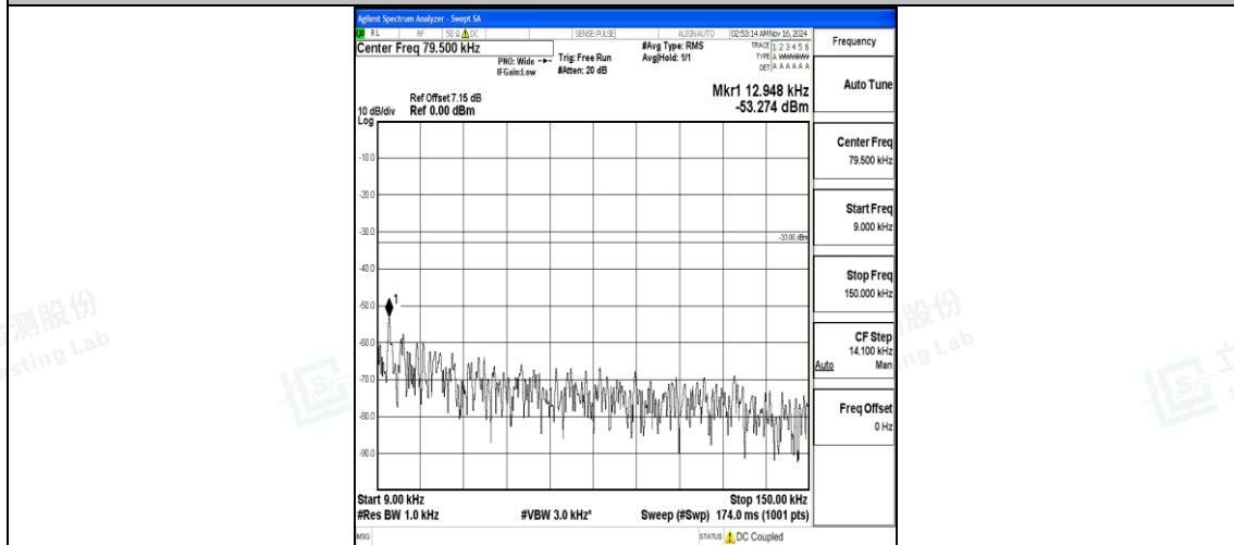
Band26_10MHz_16QAM_26990_1RB#0_0.009~0.15_0.009~0.15
