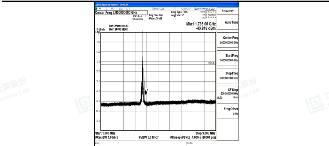
Band4_20MHz_QPSK_20175_1RB#0_1000~3000_1000~3000
