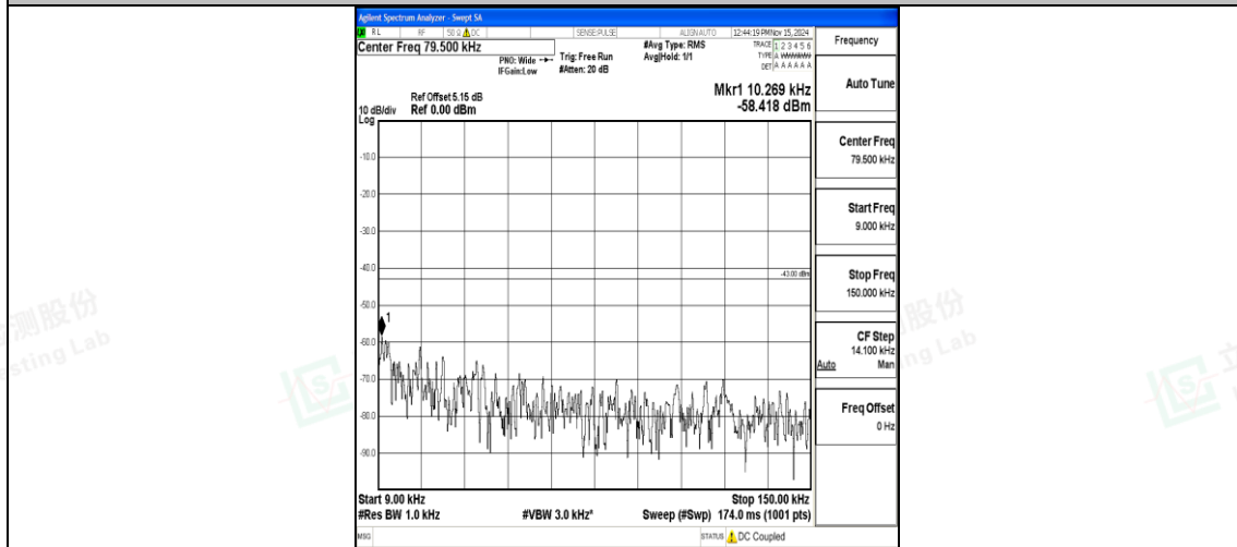
Band4_15MHz_QPSK_20175_1RB#0_0.009~0.15_0.009~0.15
