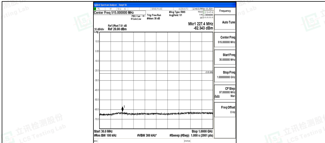
Band4_15MHz_16QAM_20325_1RB#0_30~1000_30~1000
