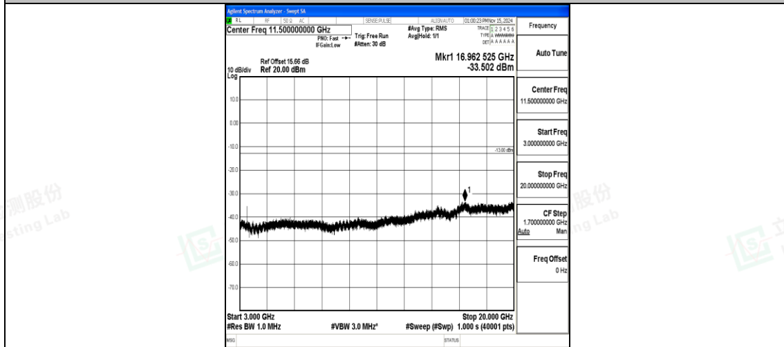
Band4_20MHz_16QAM_20175_1RB#0_3000~20000_3000~20000
