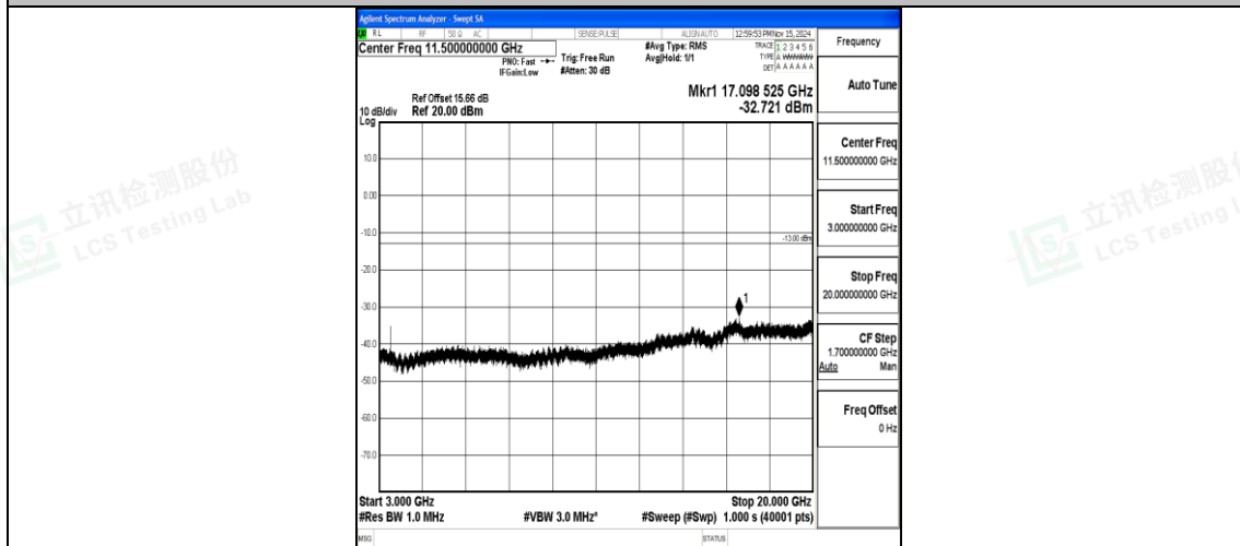
Band4_20MHz_QPSK_20175_1RB#0_3000~20000_3000~20000
