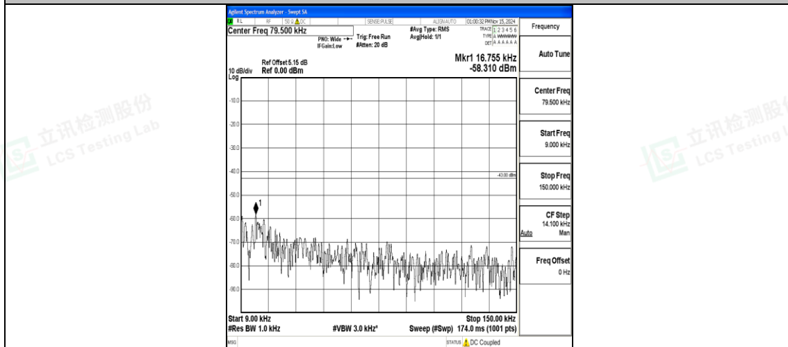
Band4_20MHz_QPSK_20300_1RB#0_0.009~0.15_0.009~0.15
