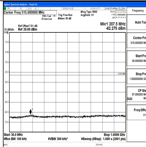
Band2_10MHz_16QAM_18650_1RB#0_30~1000_30~1000
