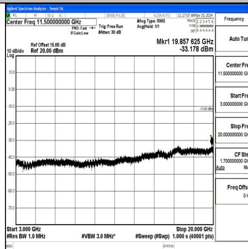
Band2_20MHz_QPSK_18900_1RB#0_3000~20000_3000~20000
