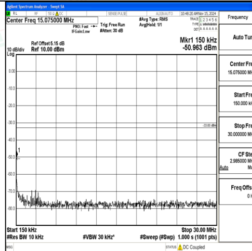
Band2_10MHz_16QAM_18650_1RB#0_0.15~30_0.15~30
