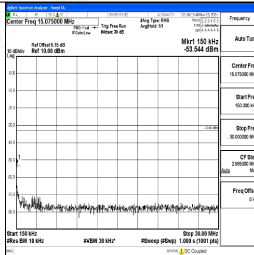
Band2_20MHz_16QAM_18700_1RB#0_0.15~30_0.15~30
