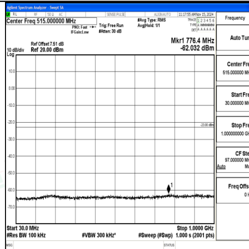
Band2_20MHz_QPSK_19100_1RB#0_30~1000_30~1000
