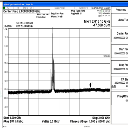
Band2_20MHz_QPSK_18900_1RB#0_1000~3000_1000~3000
