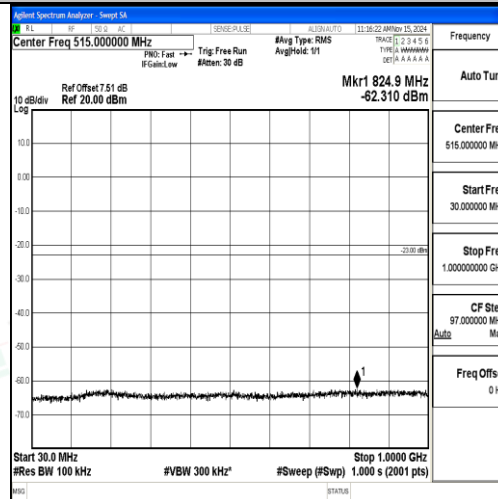
Band2_20MHz_16QAM_18700_1RB#0_30~1000_30~1000
