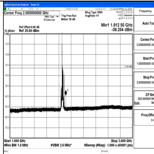
Band2_20MHz_16QAM_18700_1RB#0_1000~3000_1000~3000
