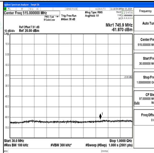
Band2_20MHz_QPSK_18900_1RB#0_30~1000_30~1000
