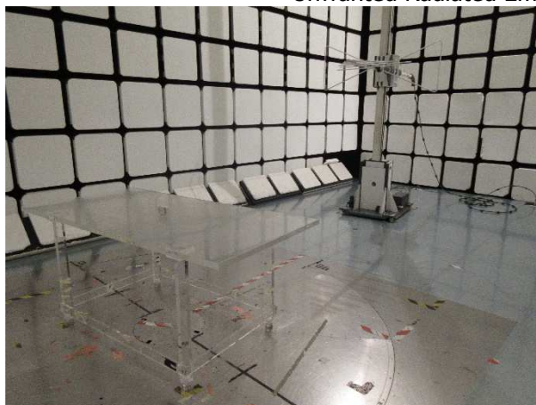
Unwanted Radiated Emission and Unwanted emissions into non-Restricted Frequency Bands (30 MHz – 1 GHz)
