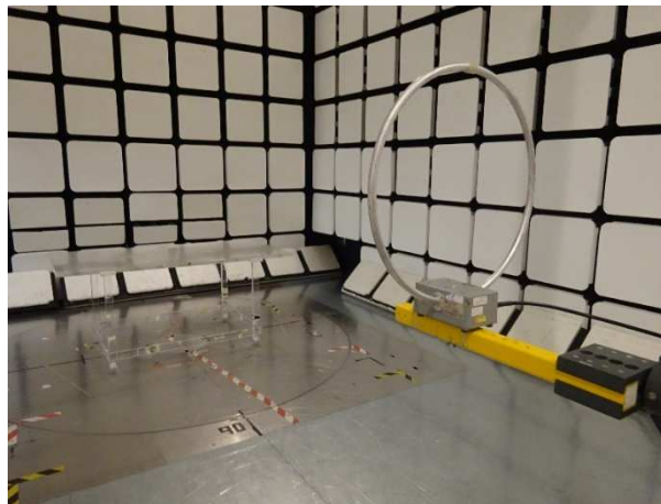
Unwanted Radiated Emission (9 kHz – 30 MHz)
