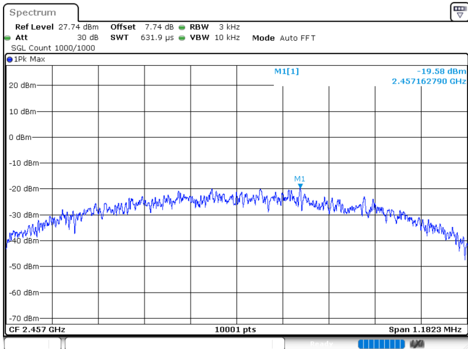
PSD NVNT ANT+ 2457MHz Ant1
