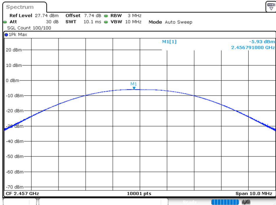
Power NVNT ANT+ 2457MHz Ant1
