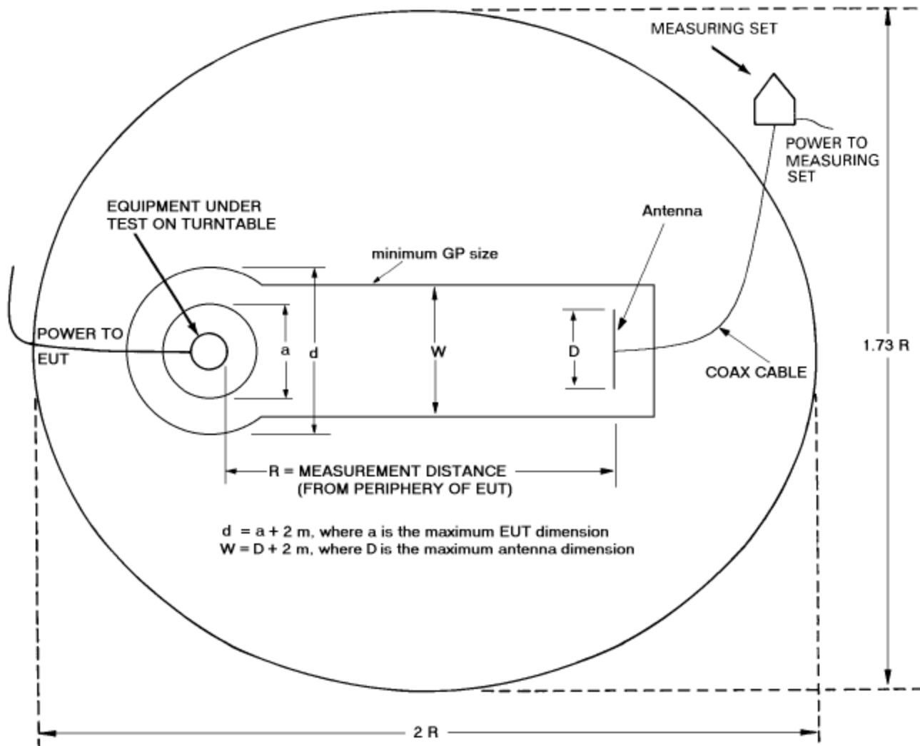
FIGURE 2: RADIATED EMISSIONS 3-METER SEMI-ANECHOIC TEST CHAMBER
