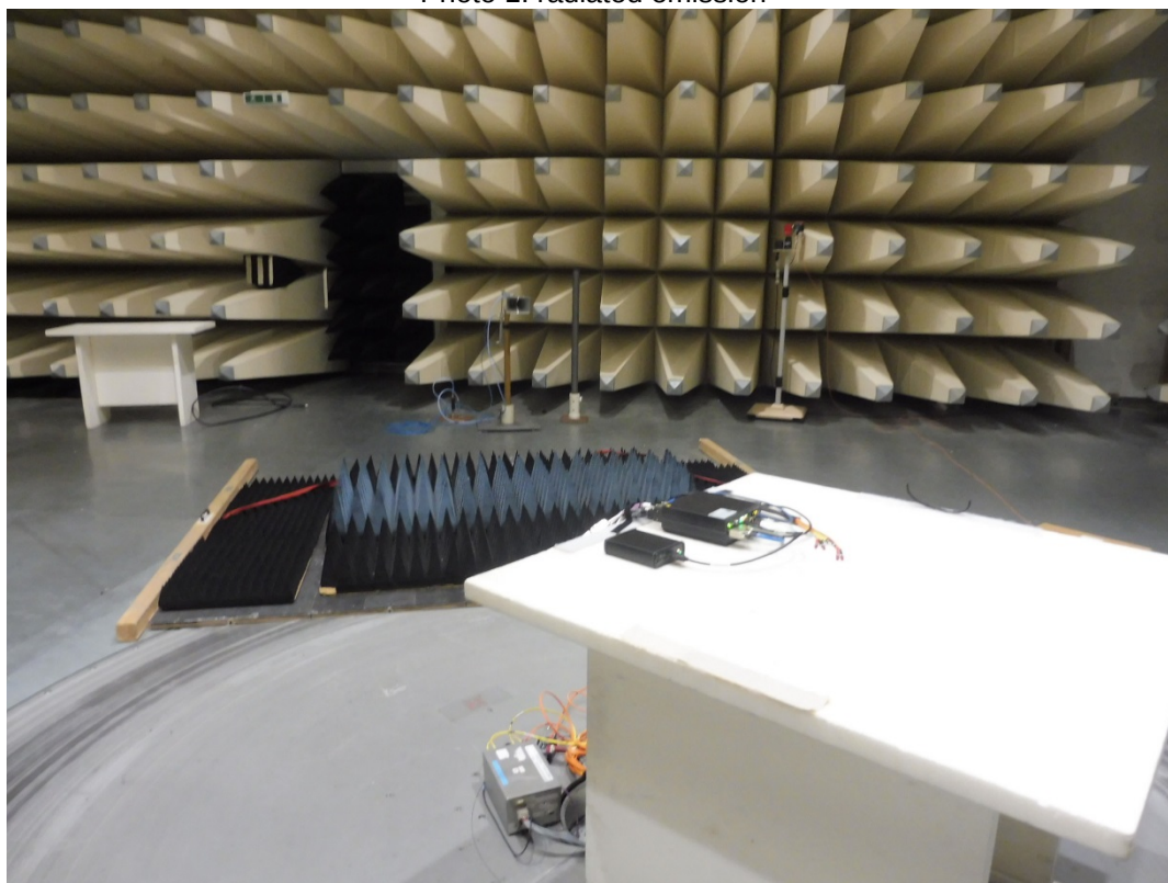
Photo 2: radiated emission
