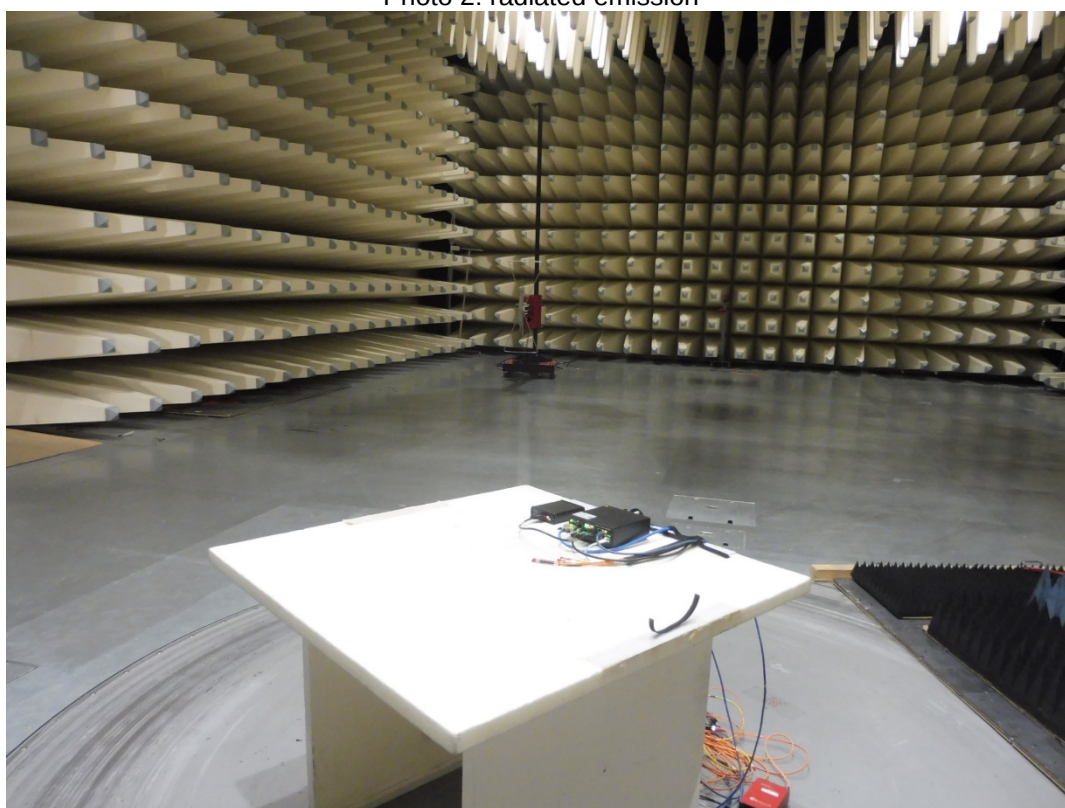
Photo 2: radiated emission
