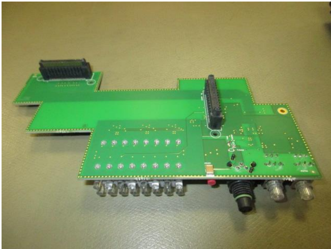
Photo 8: EUT A
