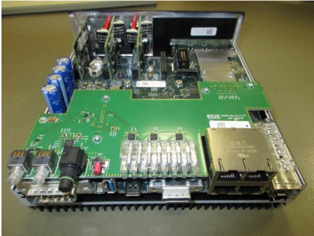
Photo 20: EUT A
