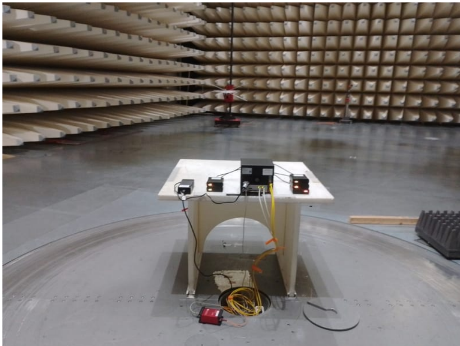
Photo 1: radiated emission <1G
