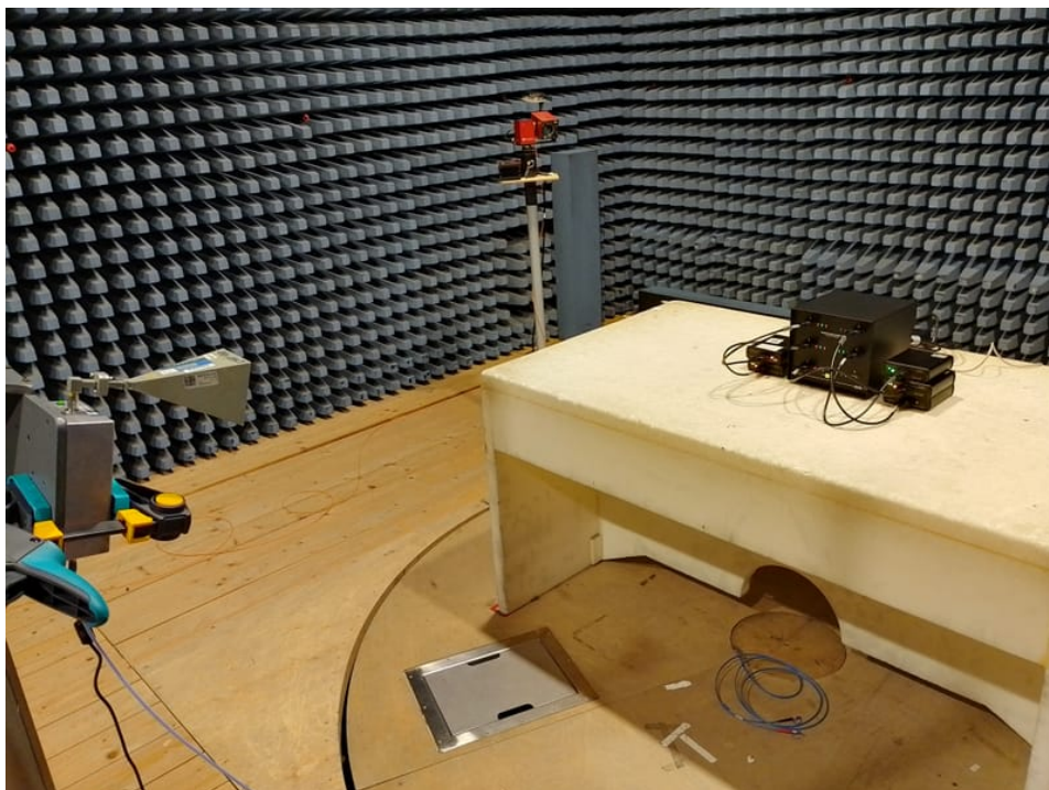
Photo 4: radiated emission 18-40G
