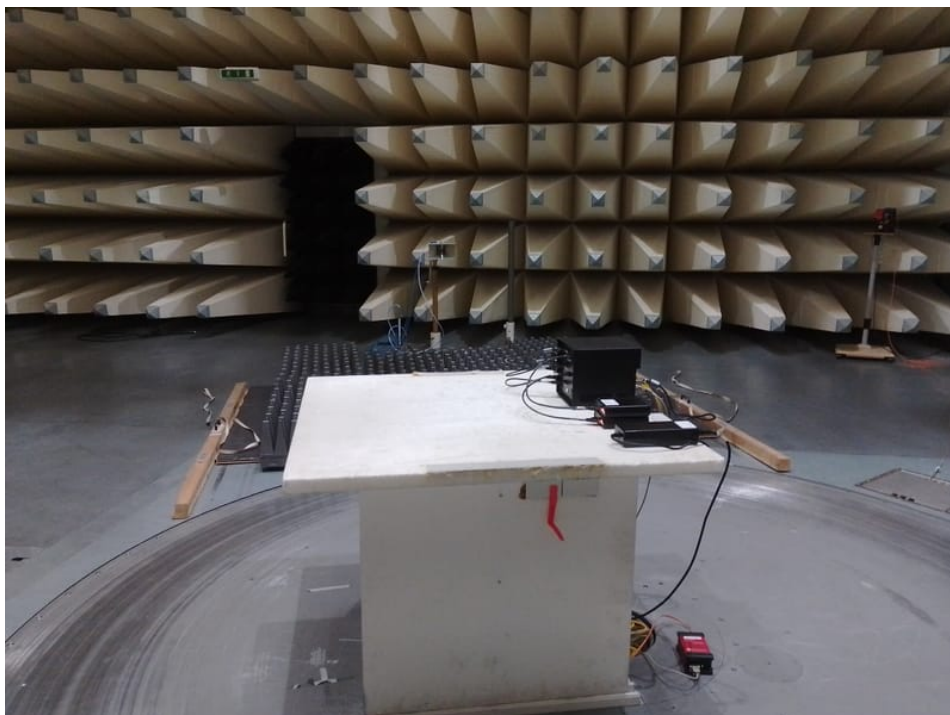
Photo 2: radiated emission >1G
