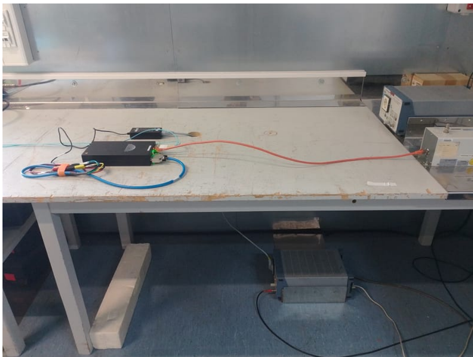
Photo 5: Set 1 conducted emission
