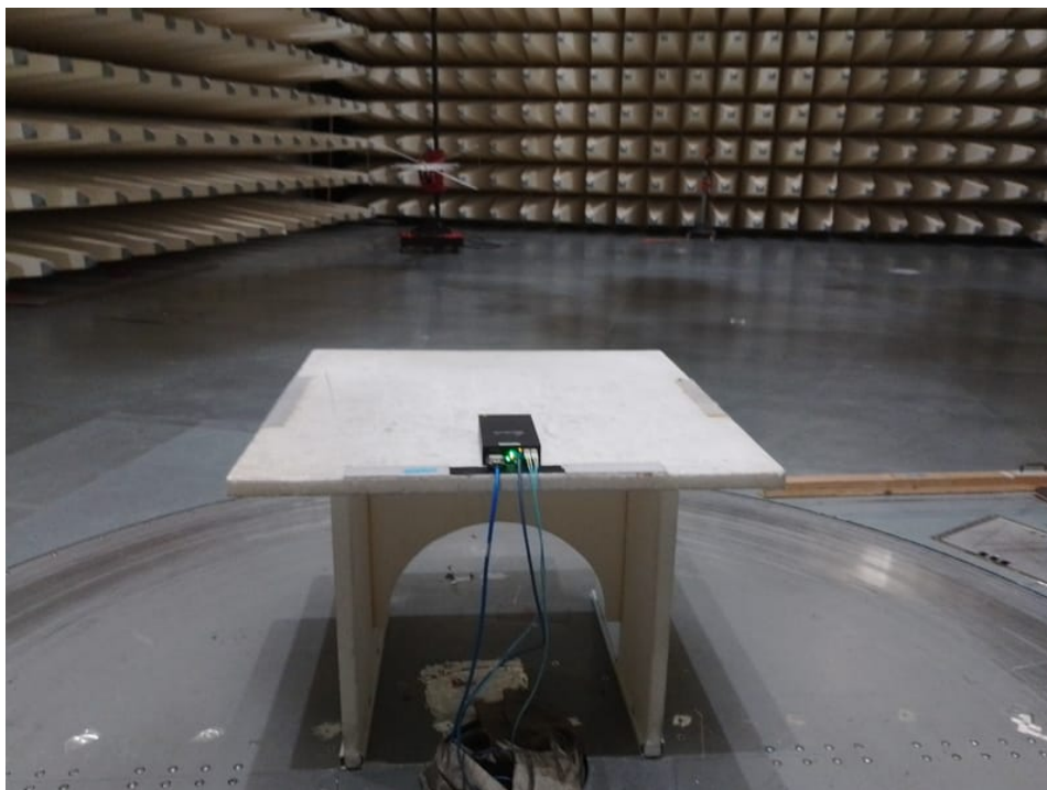
Photo 1: Set 1 Radiated emission <1G
