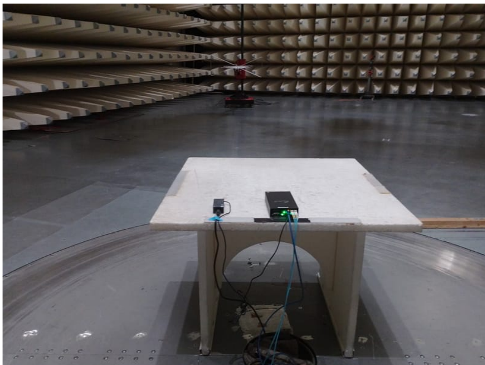
Photo 3: Set 2 Radiated emission <1G
