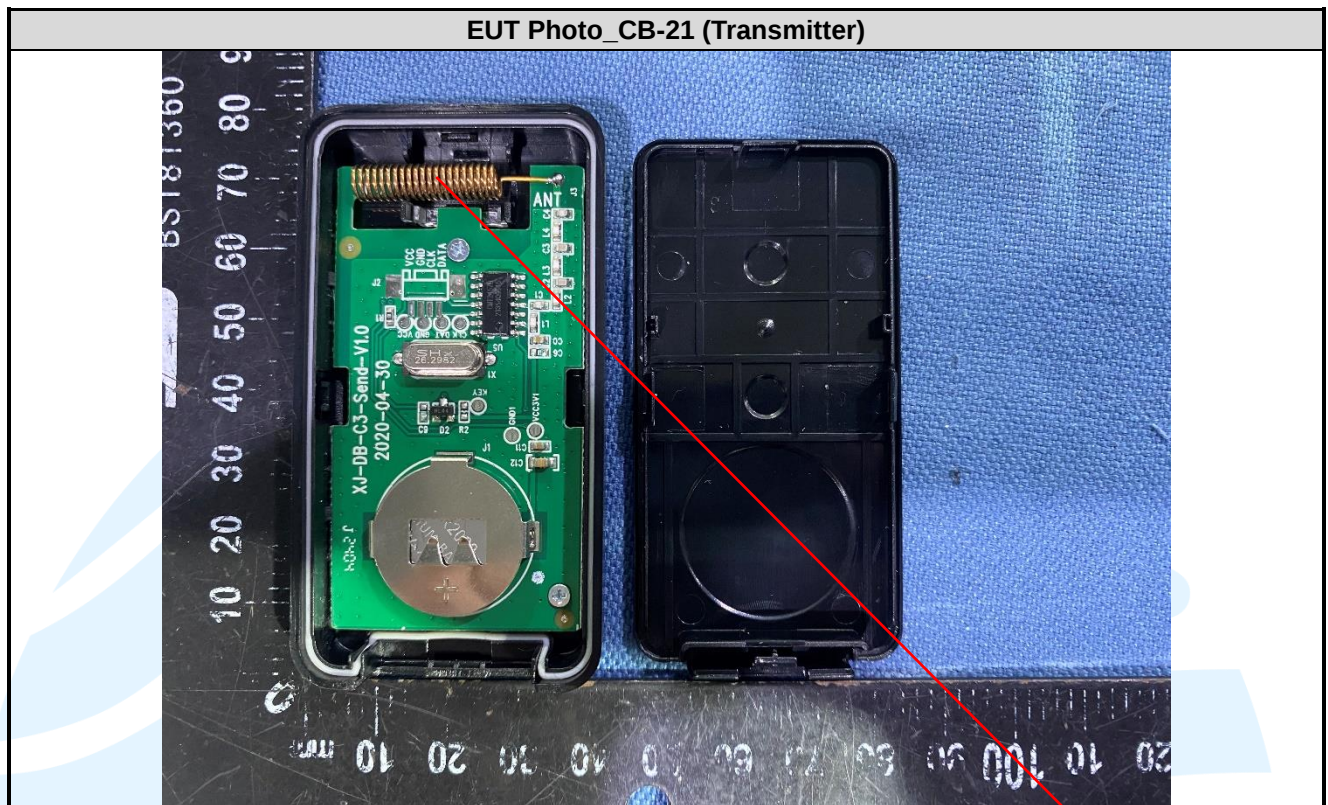
Transmitter Antenna
