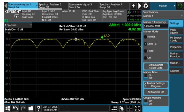
Channel 39 (2441MHz)
