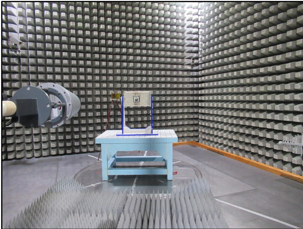
Photo 5 Radiated Test Setup-1 GHz – 18 GHz
