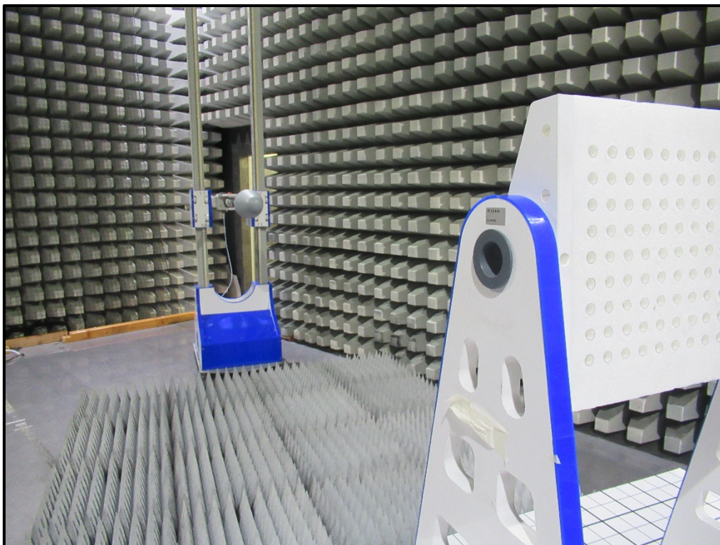
Photo 6 Radiated Test Setup-1 GHz – 18 GHz
