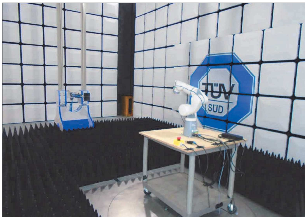
Figure 8 - Test Setup - 1 GHz to 18 GHz
