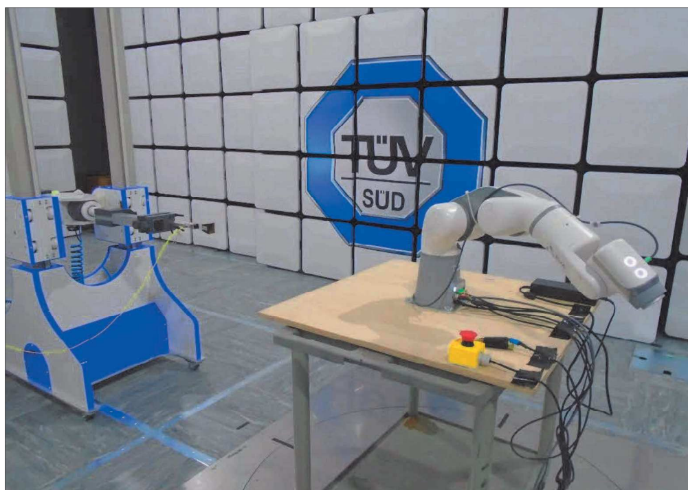
Figure 9 - Test Setup - 18 GHz to 30 GHz
