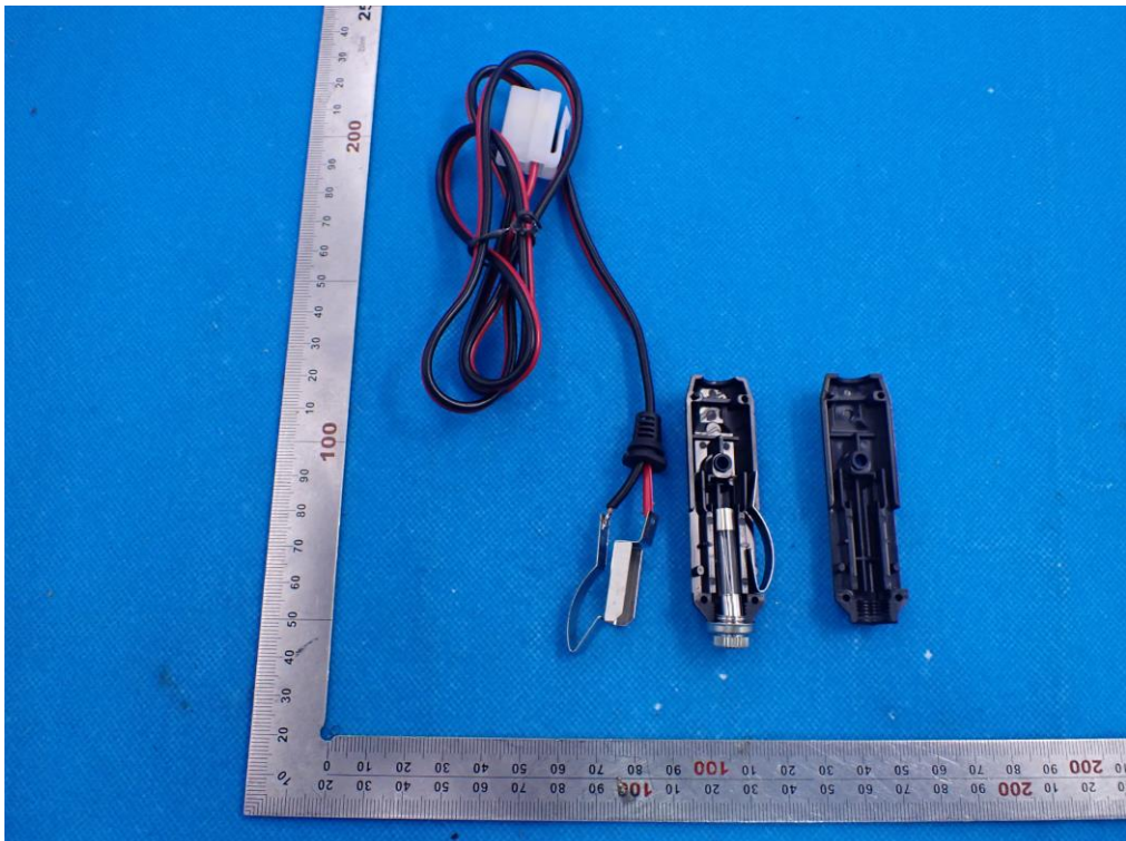
Car Charger OPEN VIEW OF EUT
