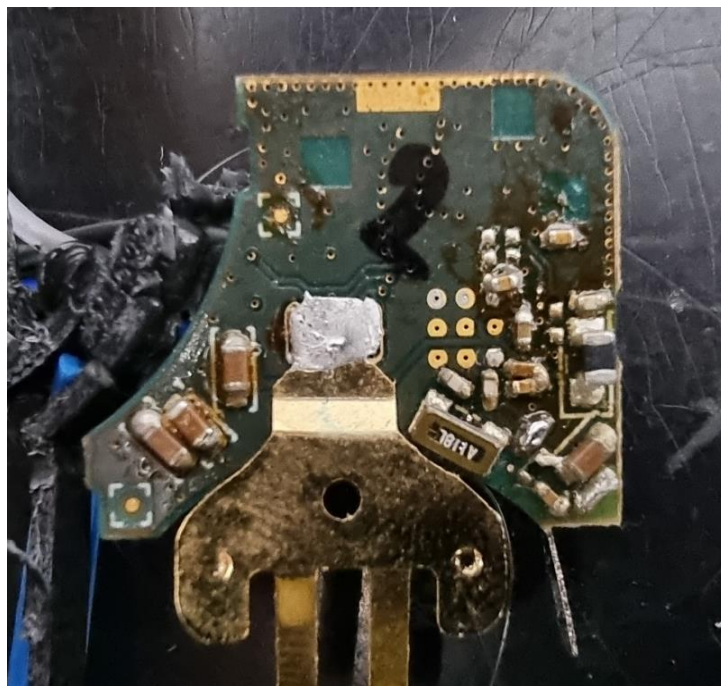
Main board - Rear Bottom
