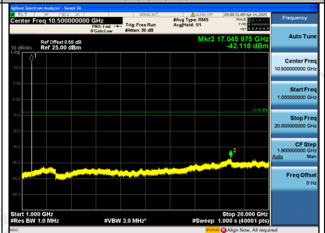
Band4-1513-1000~20000MHz-PASS
