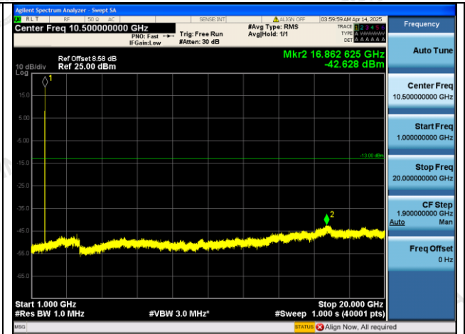
Band4-1413-1000~20000MHz-PASS
