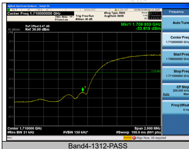
Band4-1312-PASS
