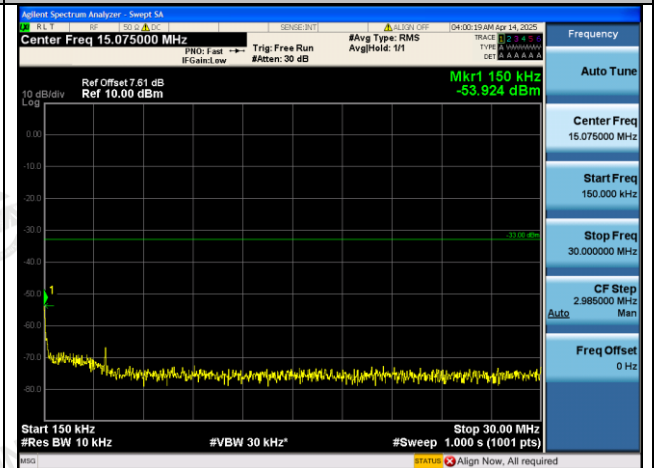
Band4-1513-0.15~30MHz-PASS
