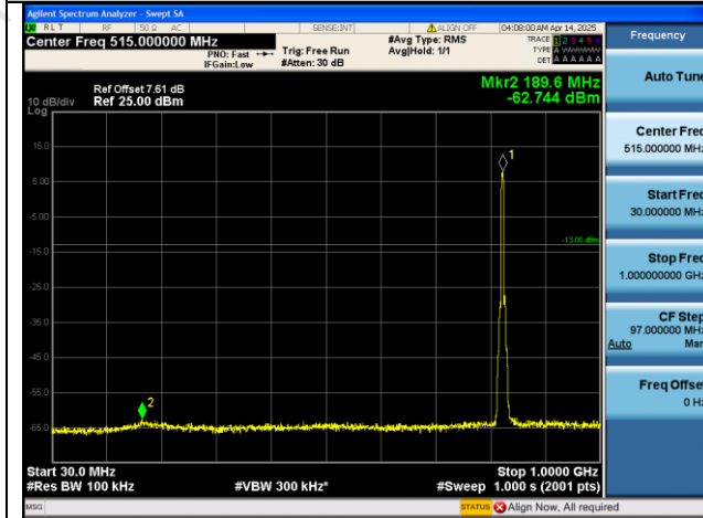
Band5-4132-30~1000MHz-PASS
