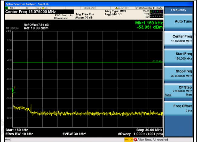
Band5-4182-0.15~30MHz-PASS
