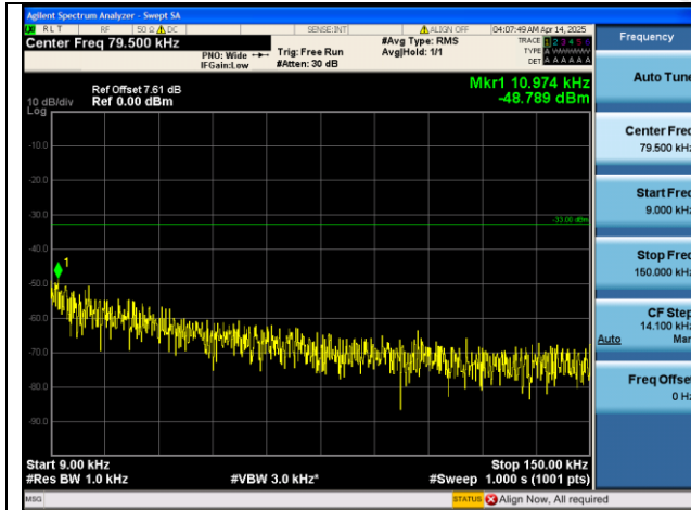
Band5-4132-0.009~0.15MHz-PASS
