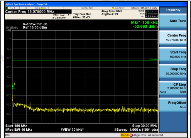
Band5-4132-0.15~30MHz-PASS
