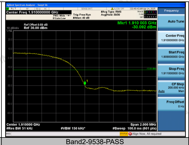
Band2-9538-PASS
