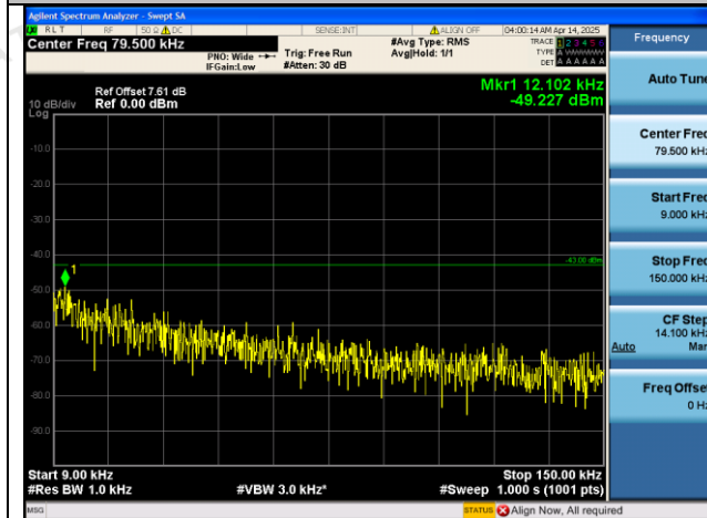
Band4-1513-0.009~0.15MHz-PASS
