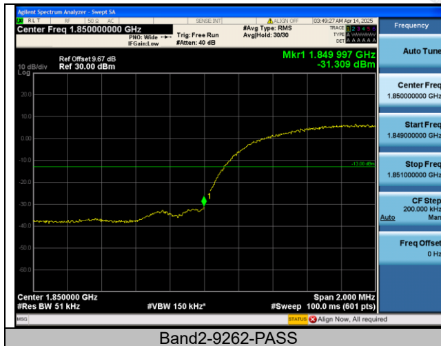
Band2-9262-PASS
