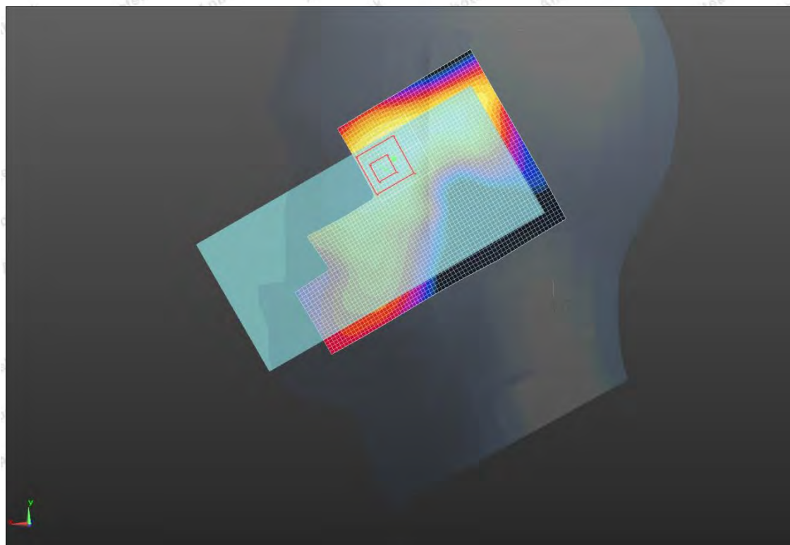
Figure 12: LTE Band 38_QPSK
