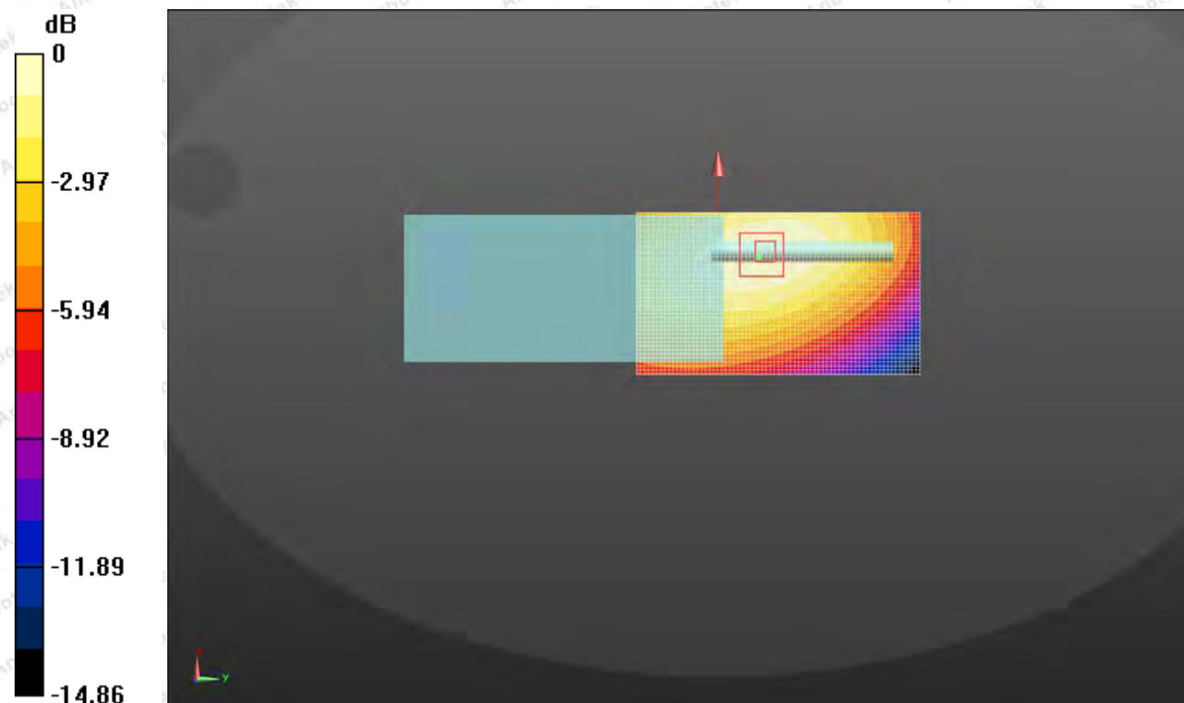
Figure 36: PMR_FM12.5KHz_Body Worn_0mm
