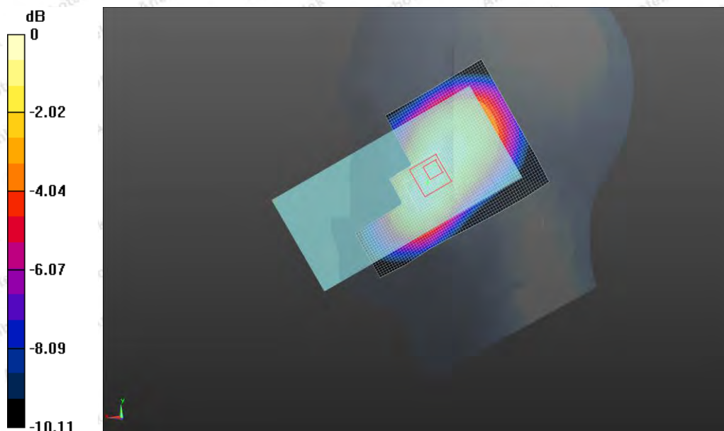
Figure 1: GSM850_GSM Voice
