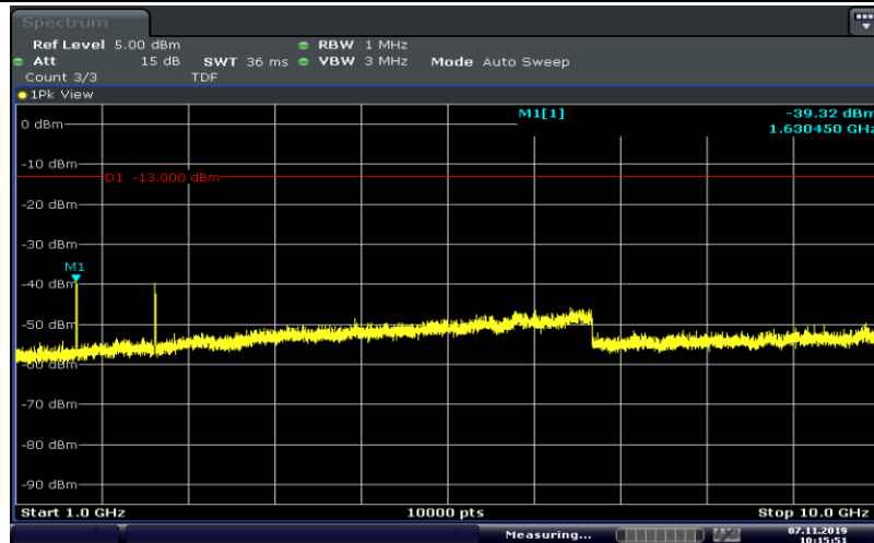
Band26-5MHz-QPSK-26715-25RB#0-Range4:1000~10000MHz
