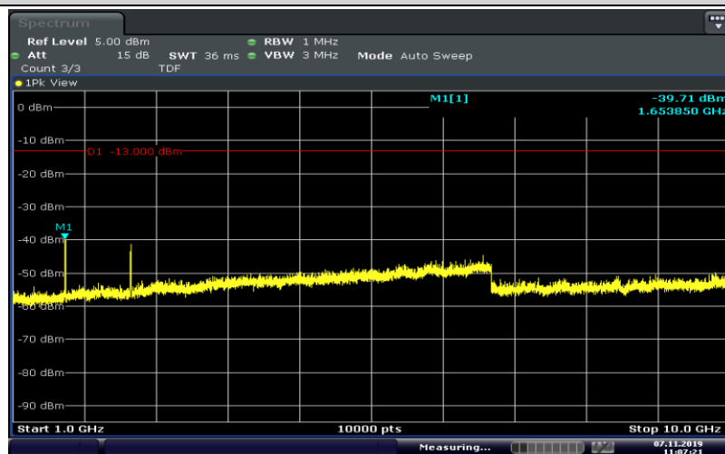
Band26-5MHz-QPSK-26815-25RB#0-Range4:1000~10000MHz
