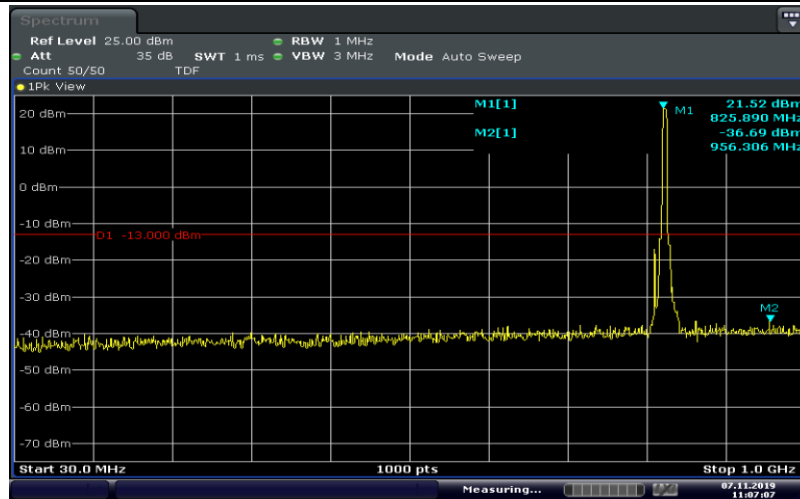
Band26-5MHz-QPSK-26815-25RB#0-Range3:30~1000MHz
