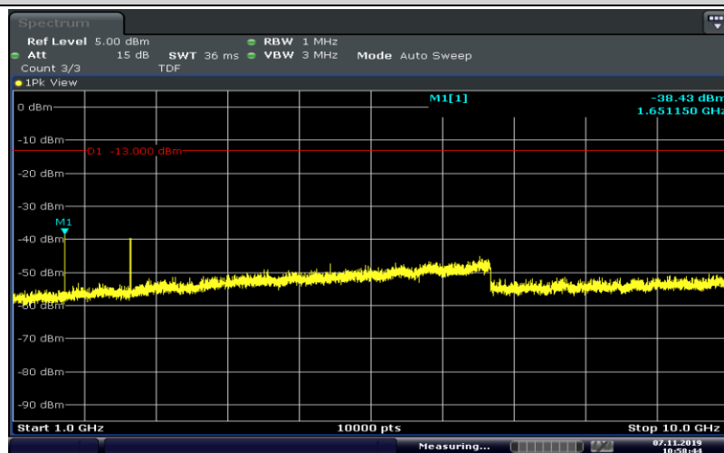
Band26-3MHz-16QAM-26805-15RB#0-Range4:1000~10000MHz
