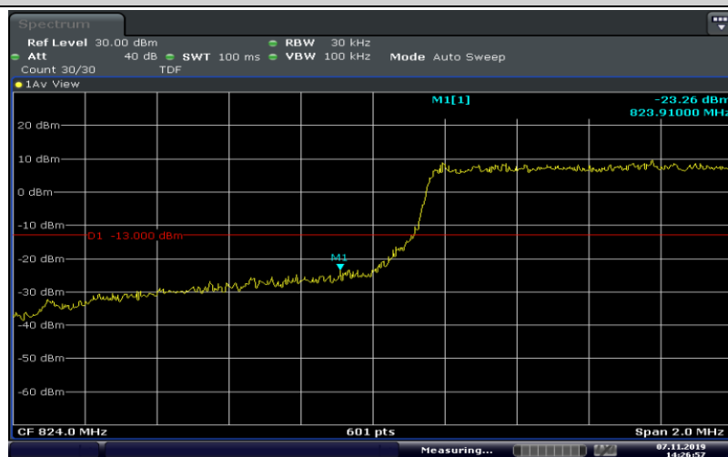
Band5-1.4MHz-16QAM-20407-6RB#0
