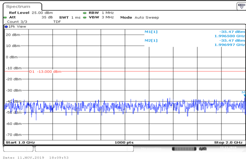
Band4-1.4MHz-16QAM-20393-6RB#0-Range4:1000~2000MHz
