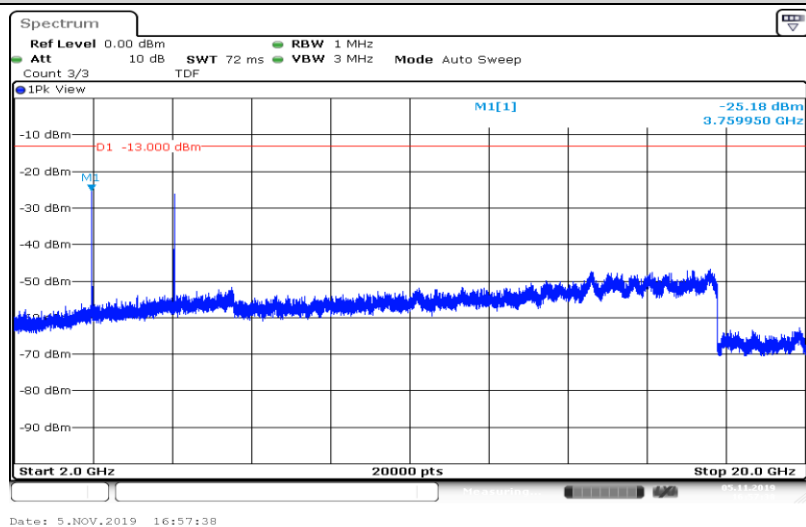
Band2-5MHz-QPSK-19175-25RB#0-Range3:30~1000MHz
