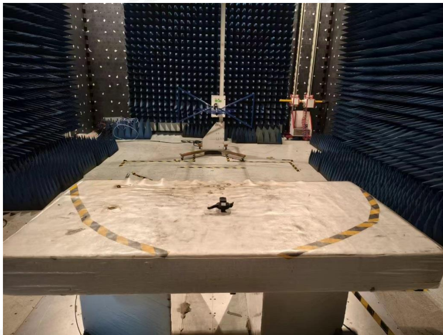
FRB radiation L
