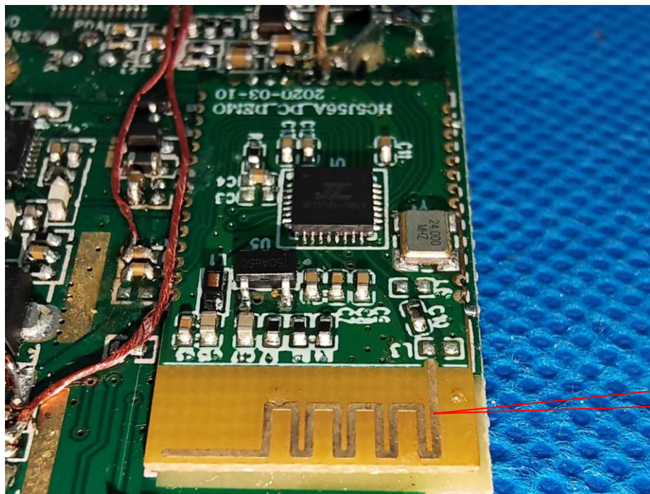
Bluetooth Antenna
