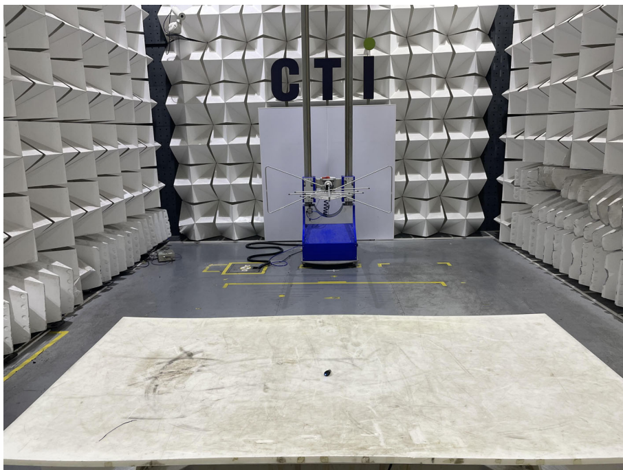
Radiated spurious emission Test Setup-1 right ears(Below 1GHz)
