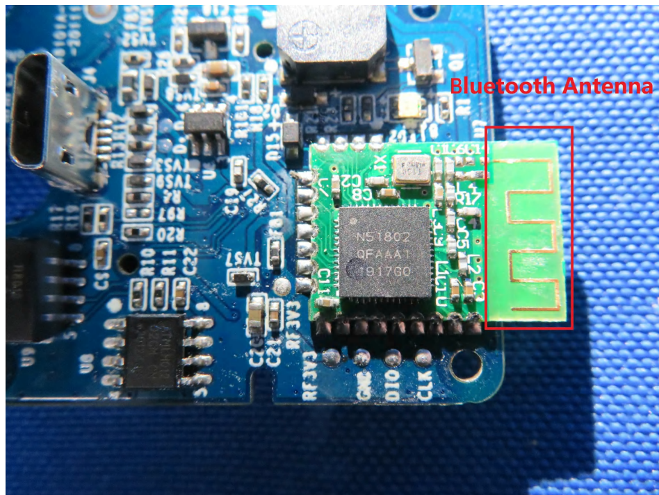
(7) EUT Photo
