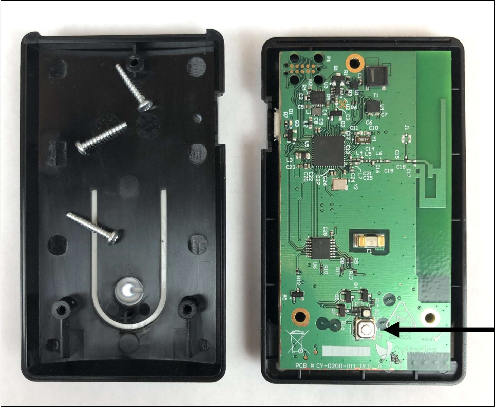
TOP Exposed
