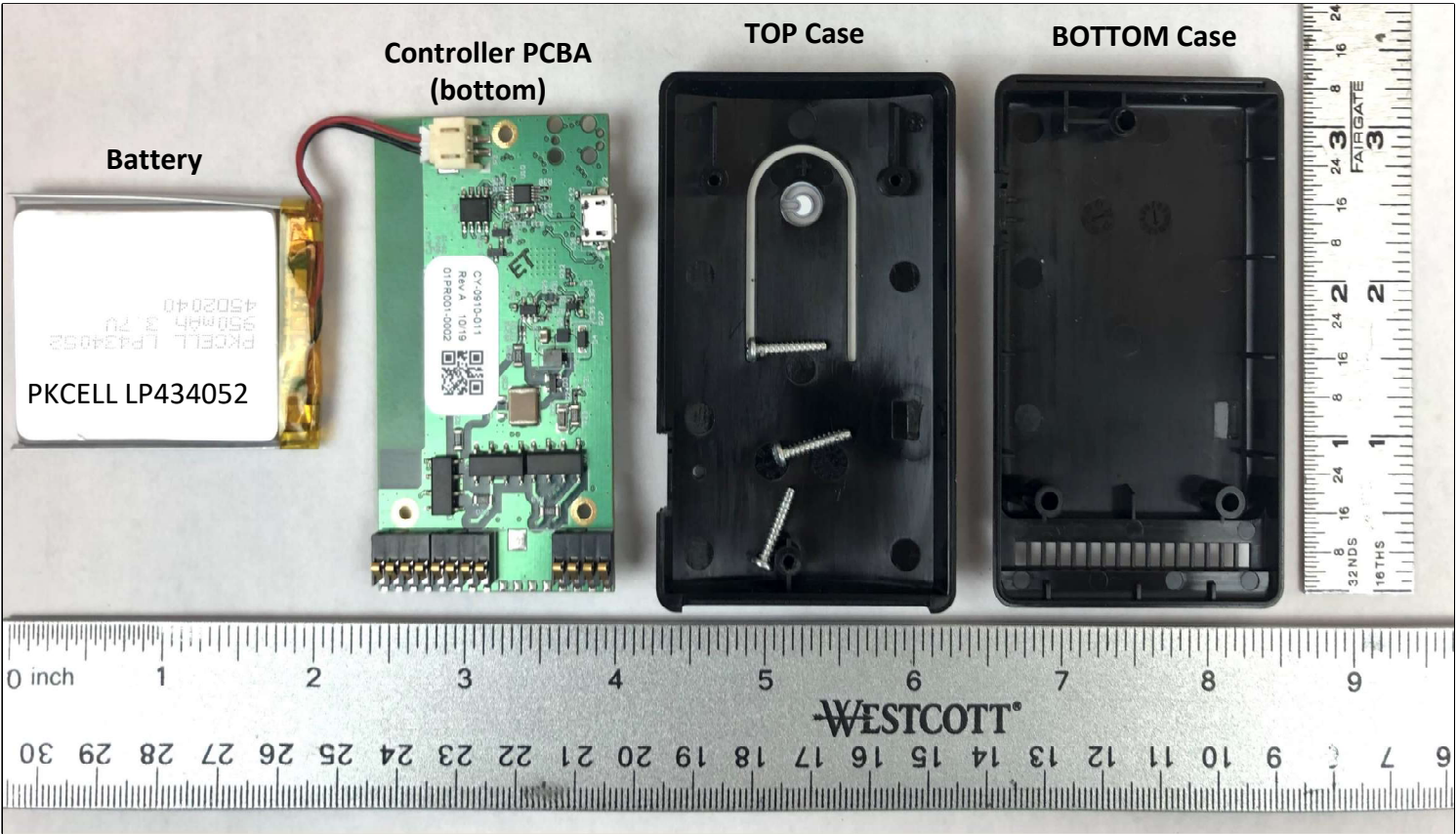
Fully Disassembled
