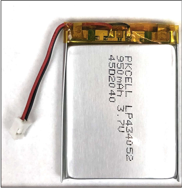
Battery - TOP
