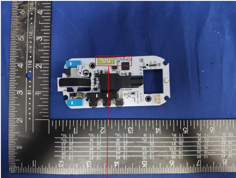
RF Antenna
