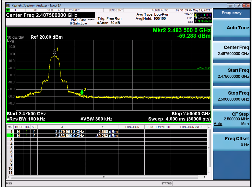
Test_Graph_EDR_ANT2_2480_2Mbps_Higher Band Edge Emissions
