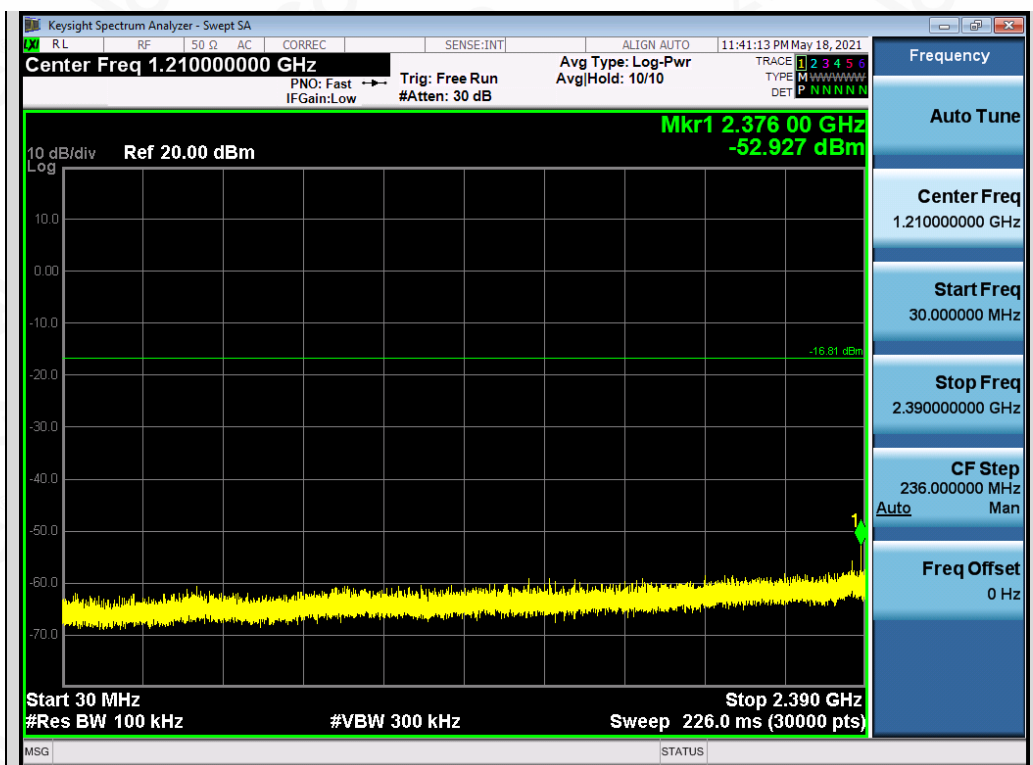
Test_Graph_BR_ANT2_2402_1Mbps_Lower Band Emissions
