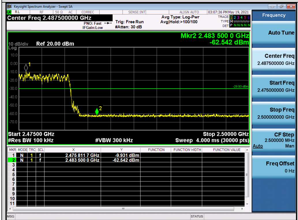
Test_Graph_EDR_HOP_ANT2_NA_3Mbps_Higher Band Edge Emissions
