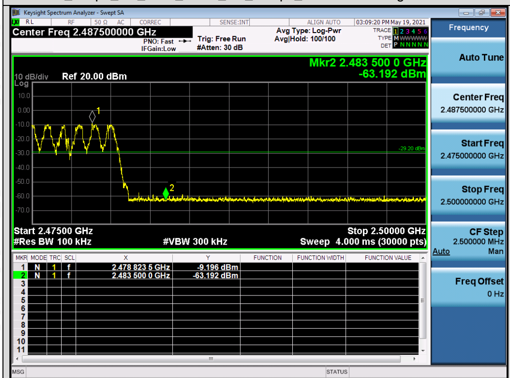
Test_Graph_BR_HOP_ANT2_NA_1Mbps_Higher Band Edge Emissions
