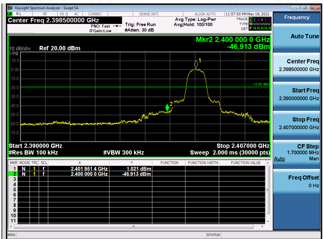
Test_Graph_EDR_ANT2_2402_2Mbps_Lower Band Edge Emissions
