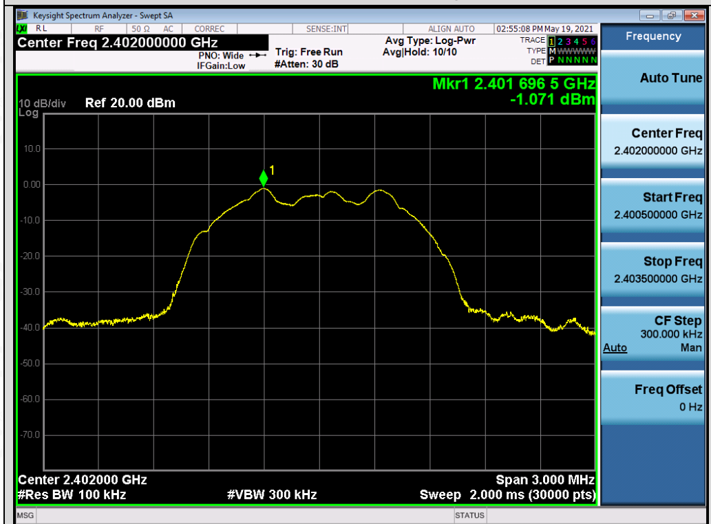
Test_Graph_EDR_ANT2_2402_3Mbps_Reference Level
