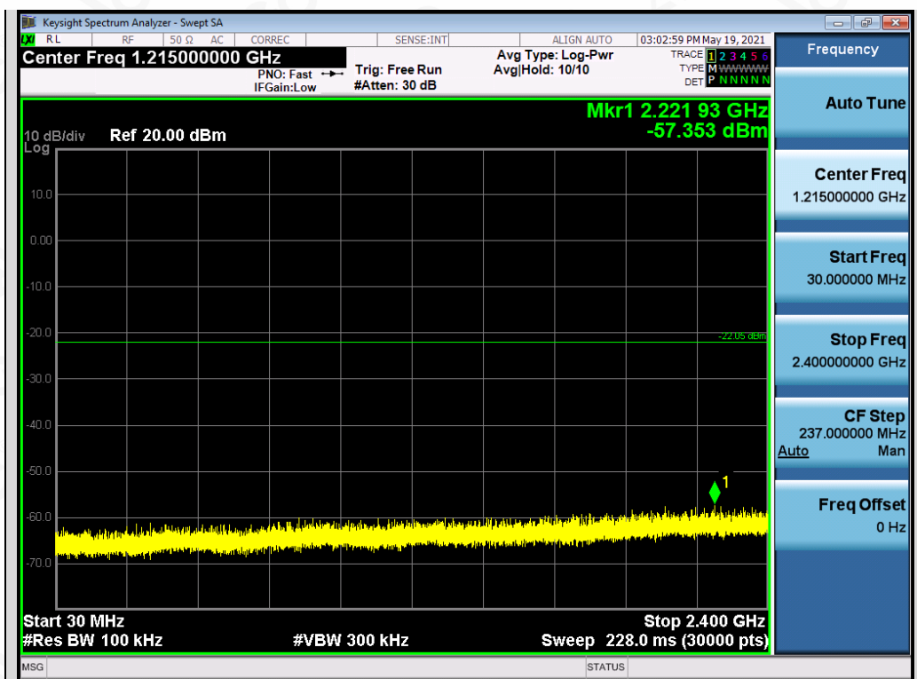
Test_Graph_EDR_ANT2_2480_3Mbps_Lower Band Emissions
