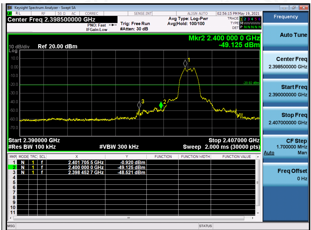
Test_Graph_EDR_ANT2_2402_3Mbps_Lower Band Edge Emissions
