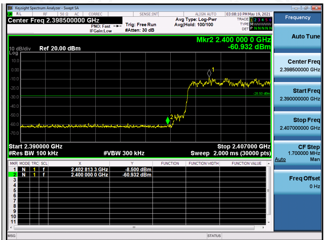
Test_Graph_EDR_HOP_ANT2_NA_2Mbps_Lower Band Edge Emissions
