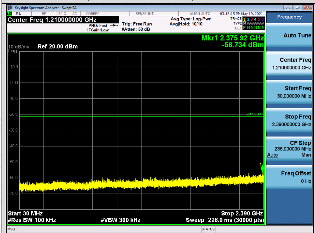
Test_Graph_EDR_ANT2_2402_2Mbps_Lower Band Emissions
