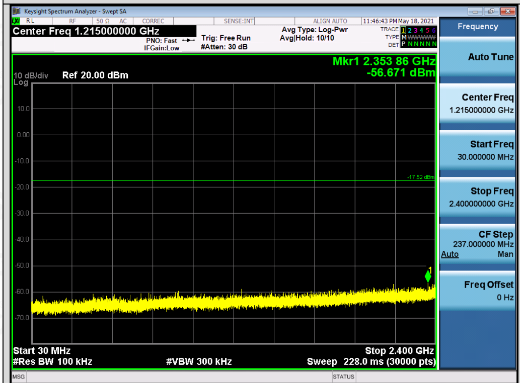
Test_Graph_BR_ANT2_2441_1Mbps_Lower Band Emissions
