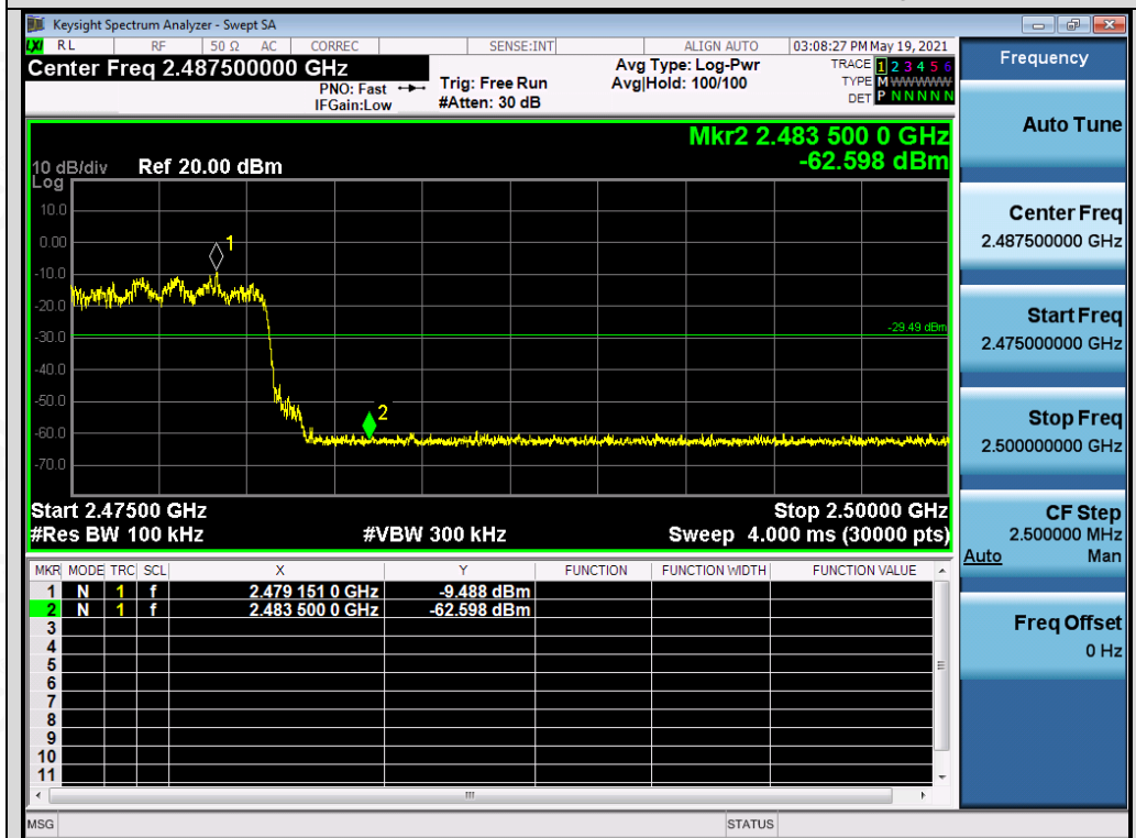
Test_Graph_EDR_HOP_ANT2_NA_2Mbps_Higher Band Edge Emissions
