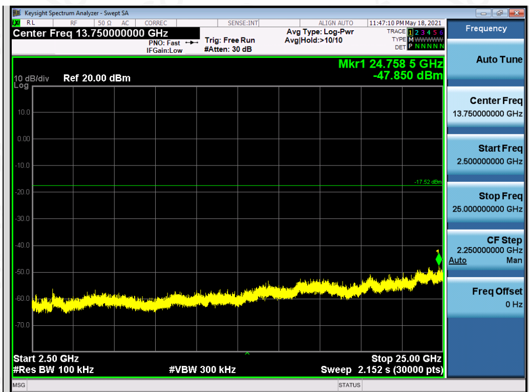
Test_Graph_BR_ANT2_2441_1Mbps_Higher Band Emissions
