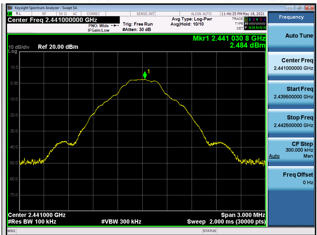
Test_Graph_BR_ANT2_2441_1Mbps_Reference Level
