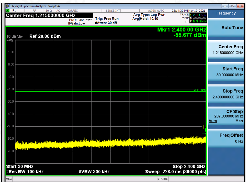
Test_Graph_EDR_ANT2_2441_2Mbps_Lower Band Emissions
