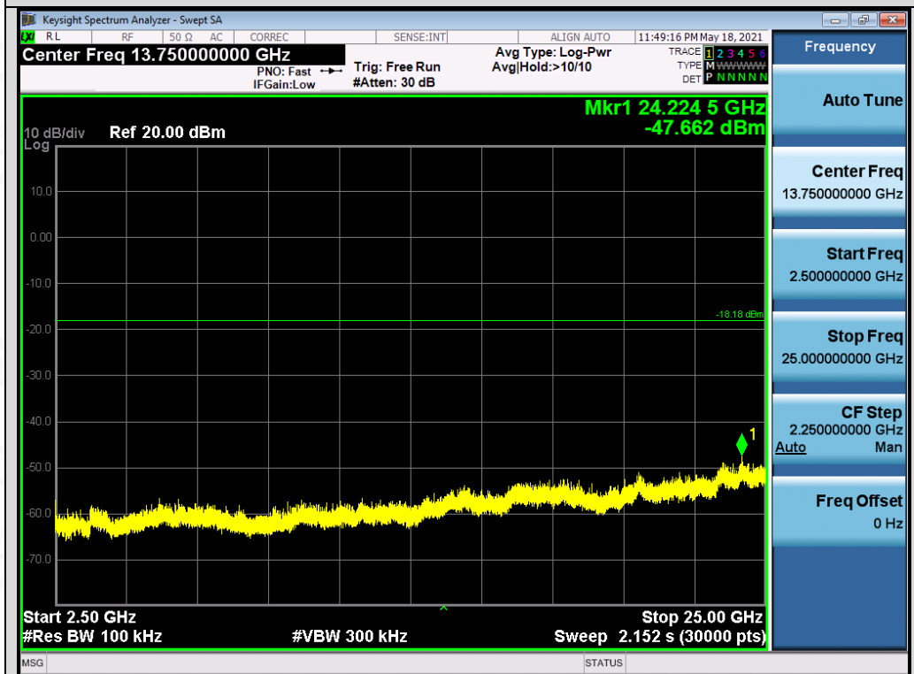
Test_Graph_BR_ANT2_2480_1Mbps_Higher Band Emissions
