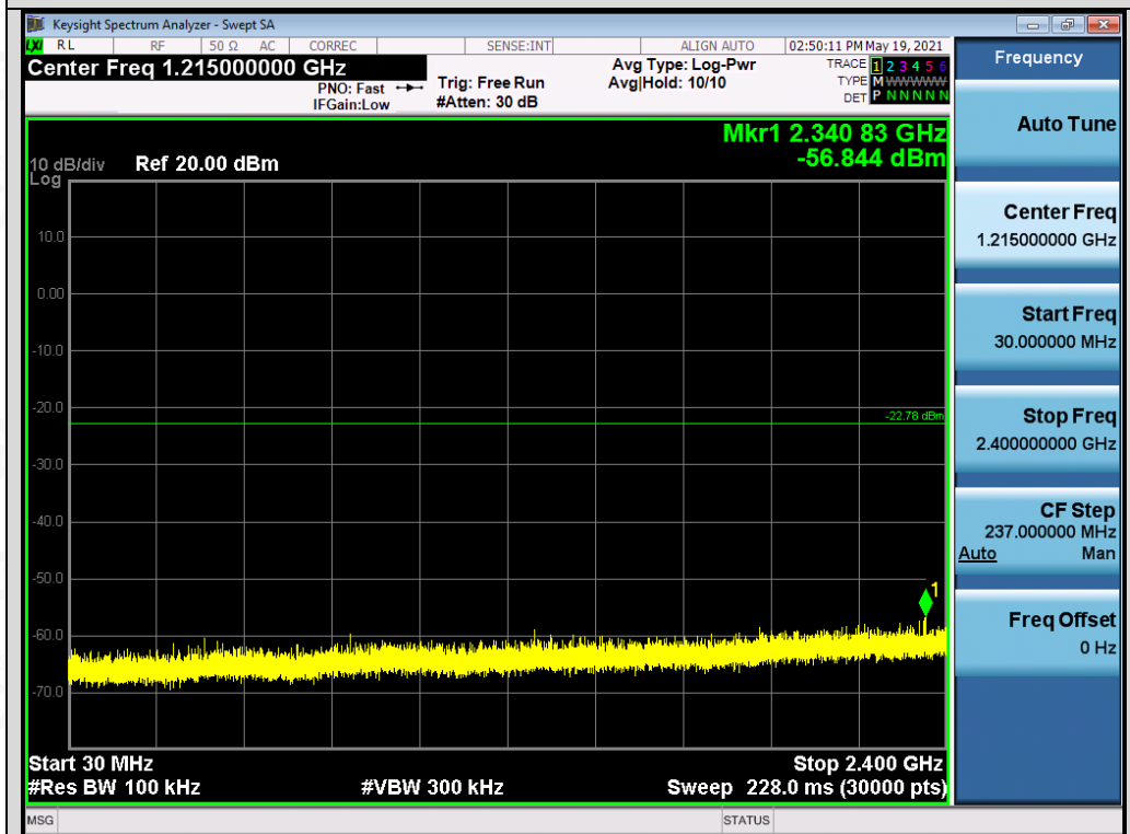
Test_Graph_EDR_ANT2_2480_2Mbps_Lower Band Emissions
