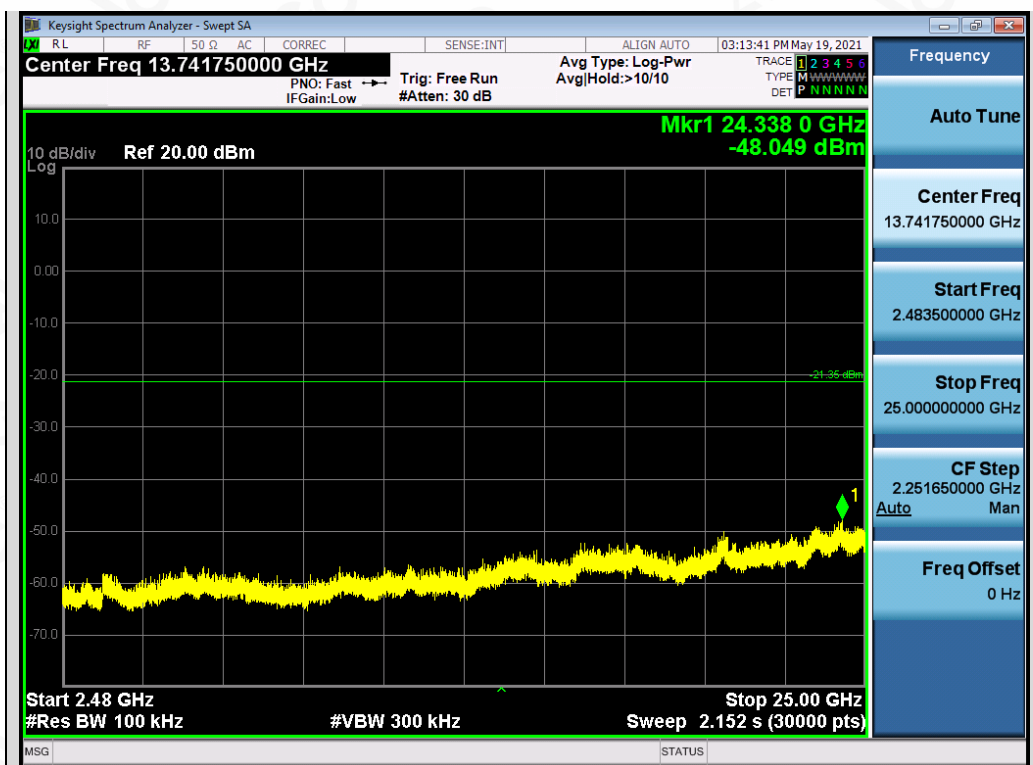
Test_Graph_EDR_ANT2_2402_2Mbps_Higher Band Emissions
