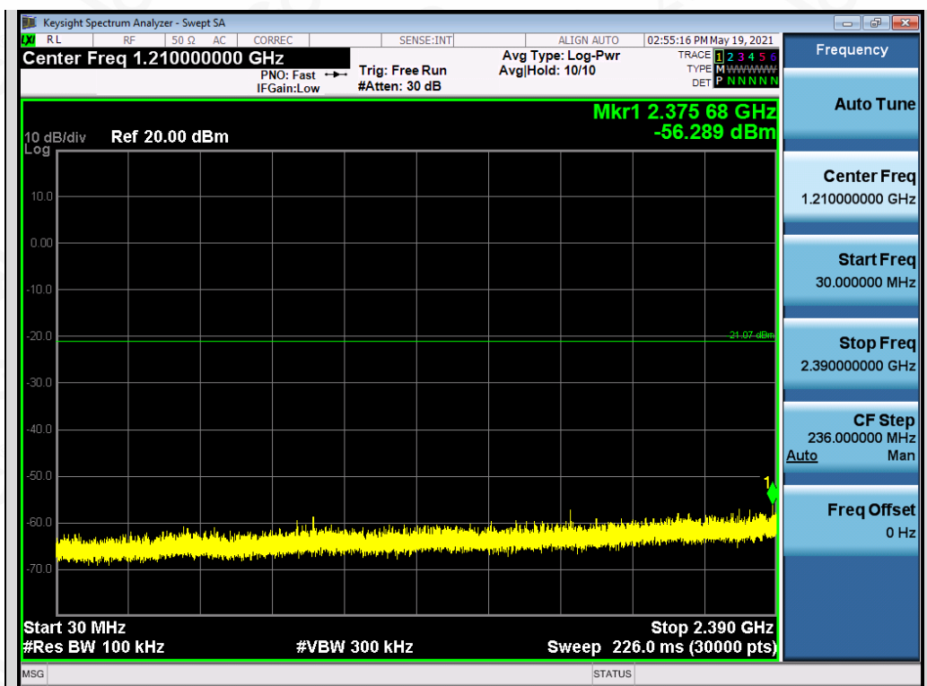
Test_Graph_EDR_ANT2_2402_3Mbps_Lower Band Emissions
