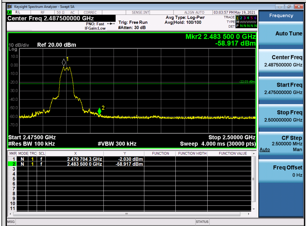
Test_Graph_EDR_ANT2_2480_3Mbps_Higher Band Edge Emissions
