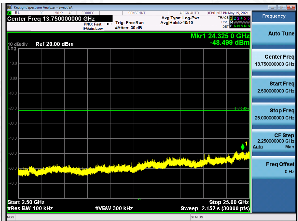
Test_Graph_EDR_ANT2_2441_3Mbps_Higher Band Emissions
