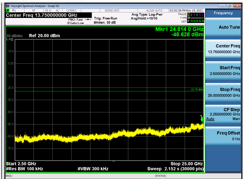
Test_Graph_EDR_ANT2_2480_2Mbps_Higher Band Emissions
