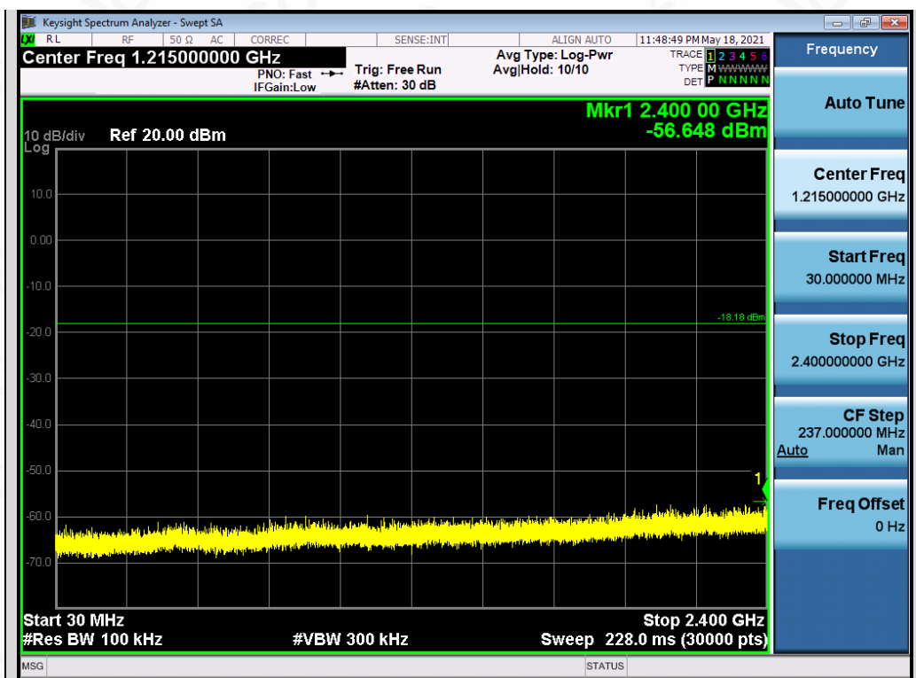
Test_Graph_BR_ANT2_2480_1Mbps_Lower Band Emissions
