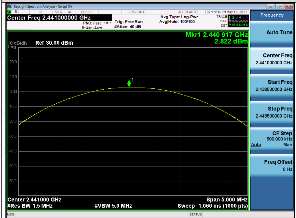
Test_Graph_EDR_ANT2_2441_2Mbps_Peak Power
