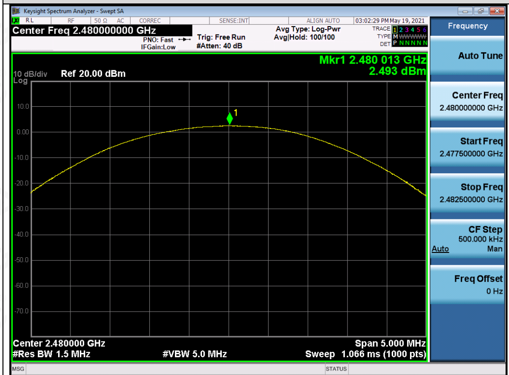
Test_Graph_EDR_ANT2_2480_3Mbps_Peak Power
