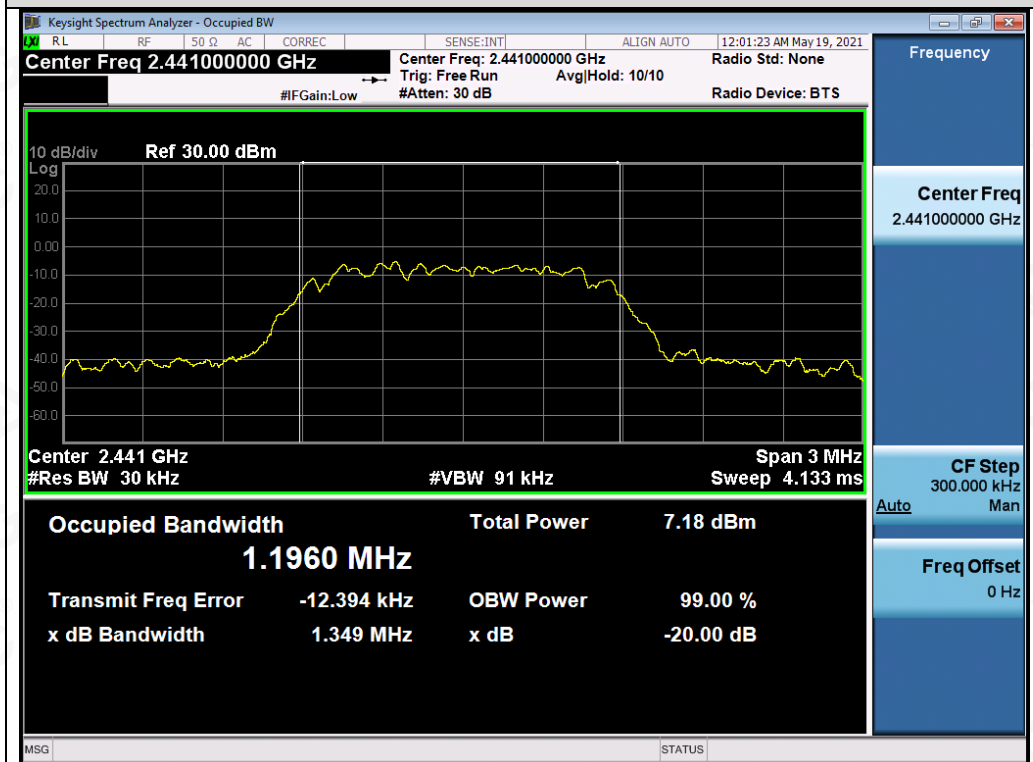
Test_Graph_EDR_ANT2_2441_2Mbps_OBW
