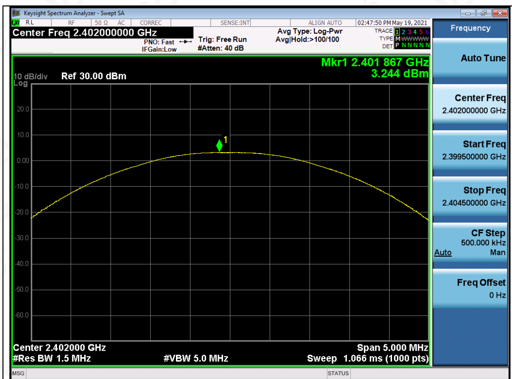
Test_Graph_EDR_ANT2_2402_2Mbps_Peak Power
