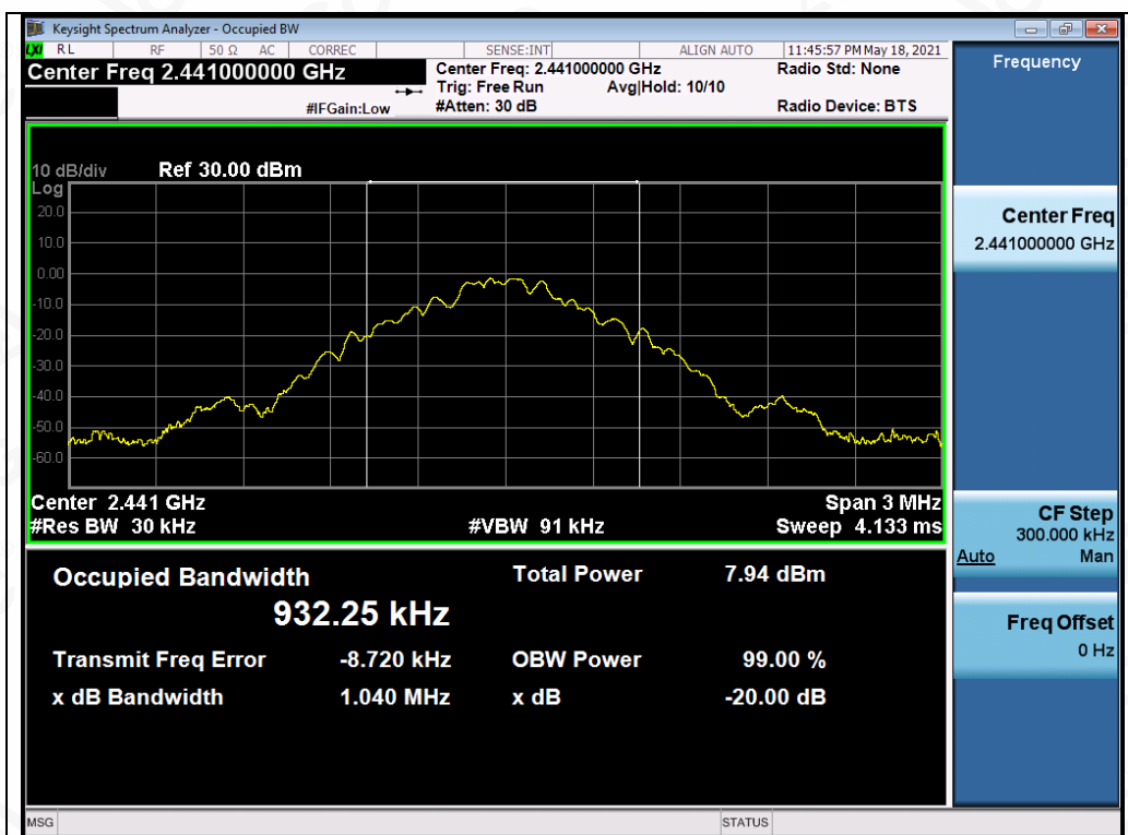
Test_Graph_BR_ANT2_2441_1Mbps_OBW
