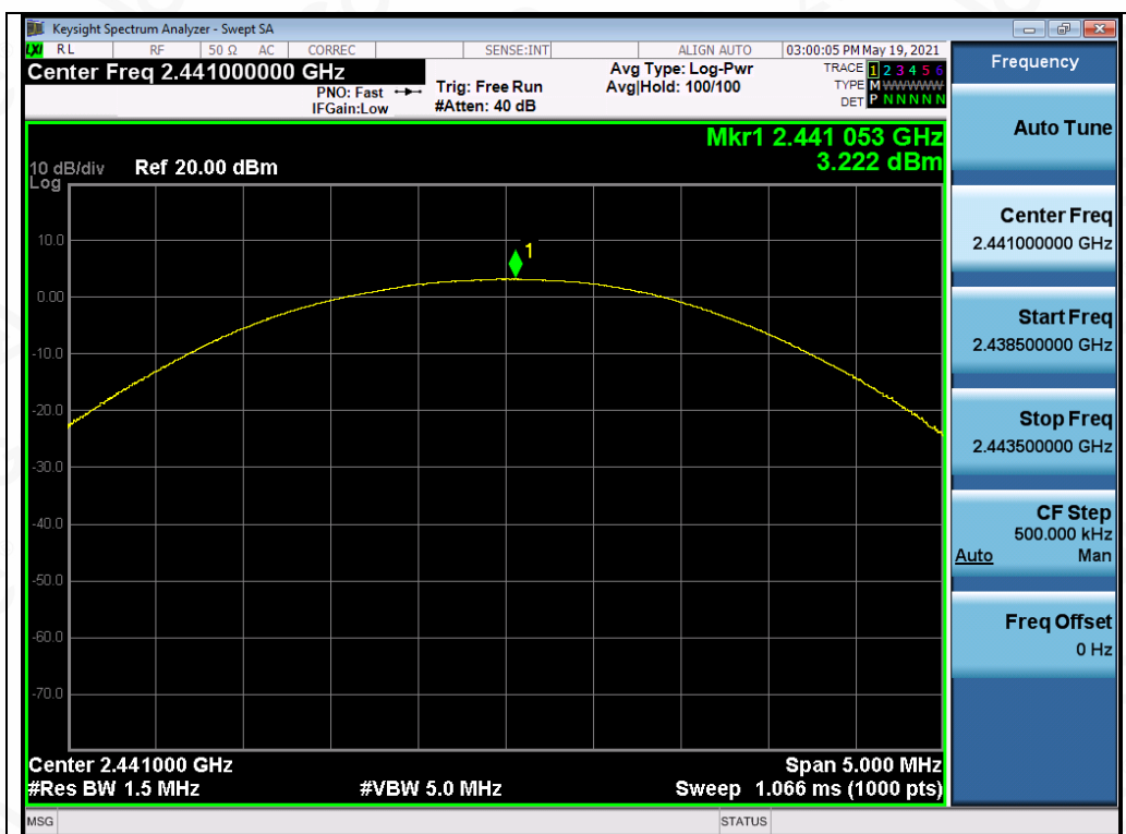
Test_Graph_EDR_ANT2_2441_3Mbps_Peak Power
