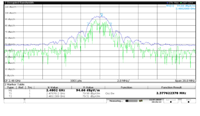
802.15.4: 99% bandwidth on Channel 26
