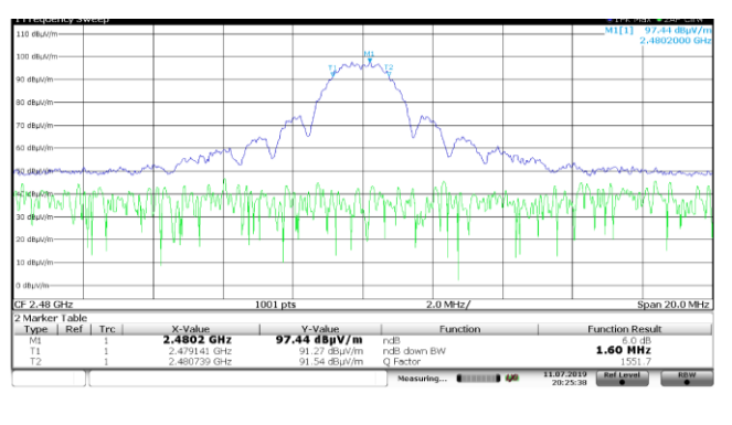
802.15.4: 6 dB bandwidth on Channel 26
