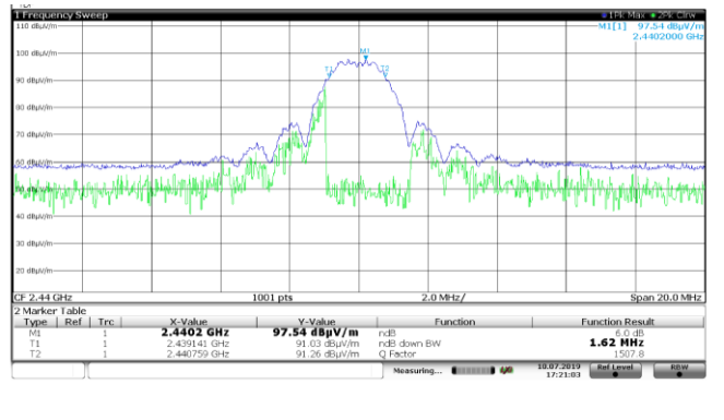
802.15.4: 6 dB bandwidth on Channel 18
