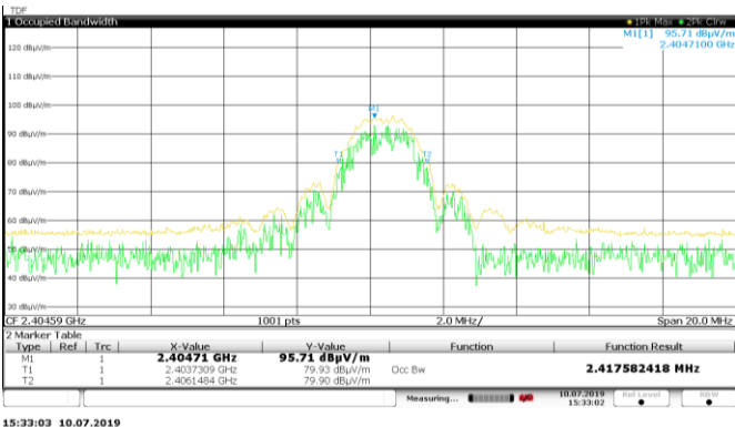
802.15.4: 99% bandwidth on Channel 11
