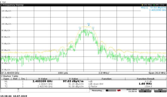
802.15.4 : 6 dB bandwidth on Channel 11
