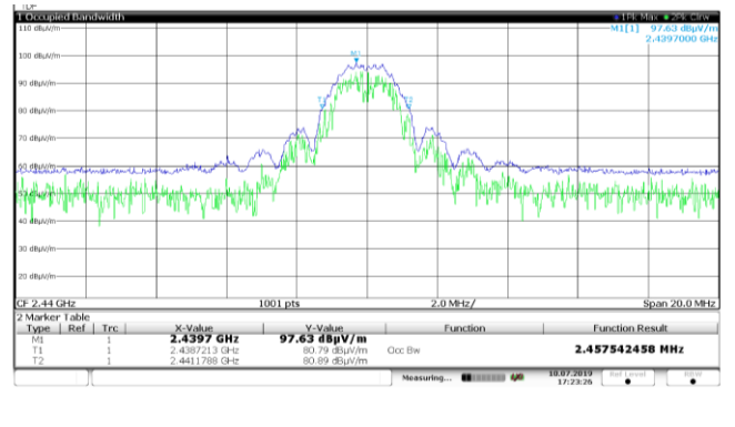
802.15.4 99% bandwidth on Channel 18
