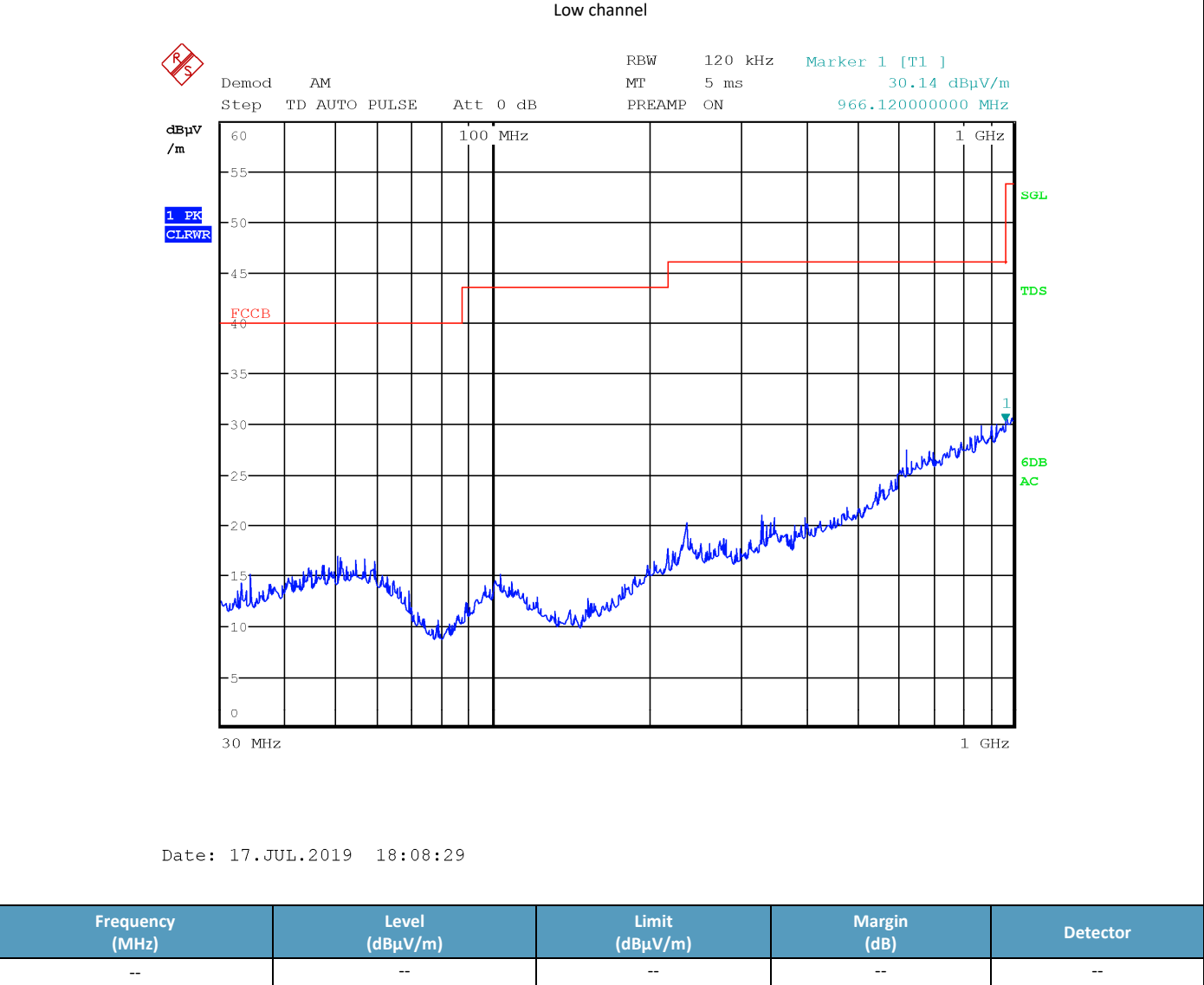
Section 8 Radiated measurement horizontal polarization, low channel
