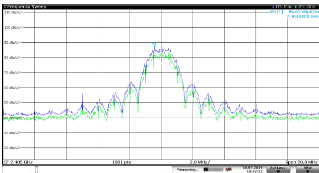
Low channel, vertical polarization
