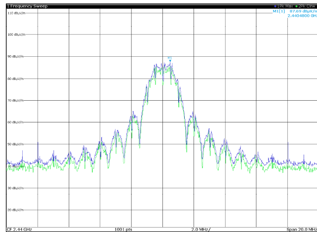
Middle channel, horizontal polarization
