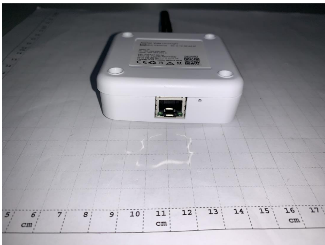
Photograph 5: EUT A, rear view
