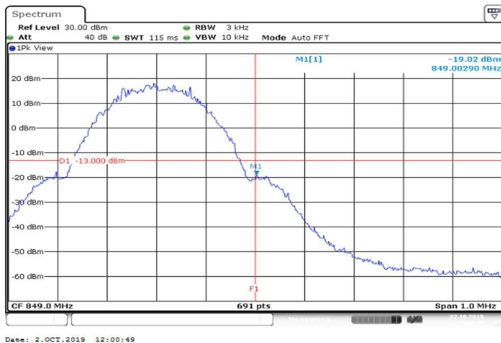
Figure 10-2: Band Edge emissions –GPRS CH High
