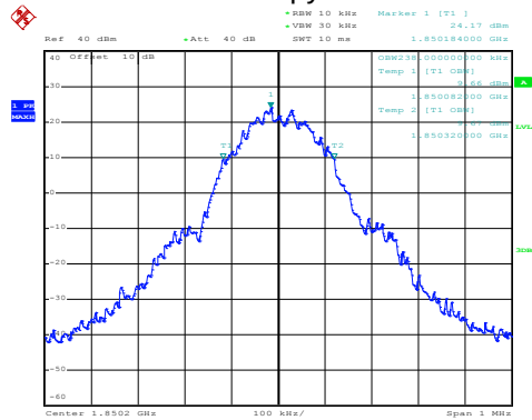
99% Occupancy bandwidth
