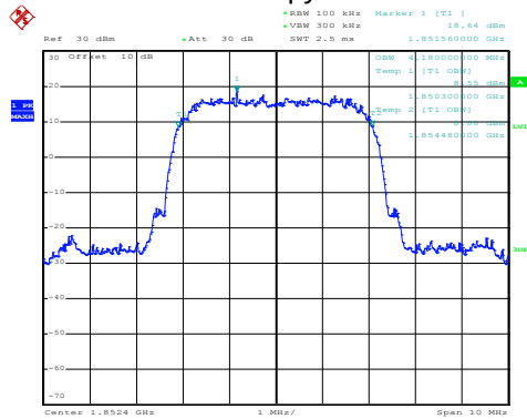
99% Occupancy bandwidth
