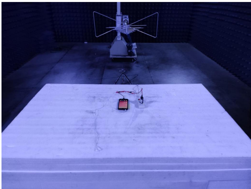
Photo of Radiated Emission Measurement (30M-1G)
