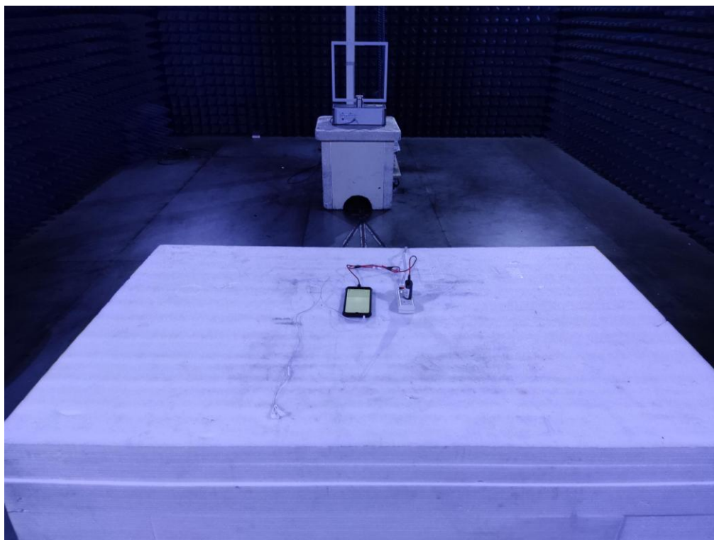
Photo of Radiated Emission Measurement (9k-30M)
