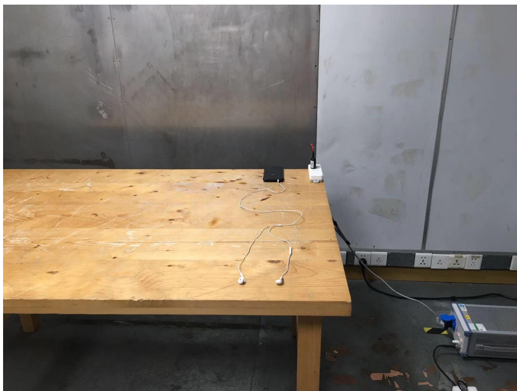
Photo of Conducted Emission Measurement – Front
