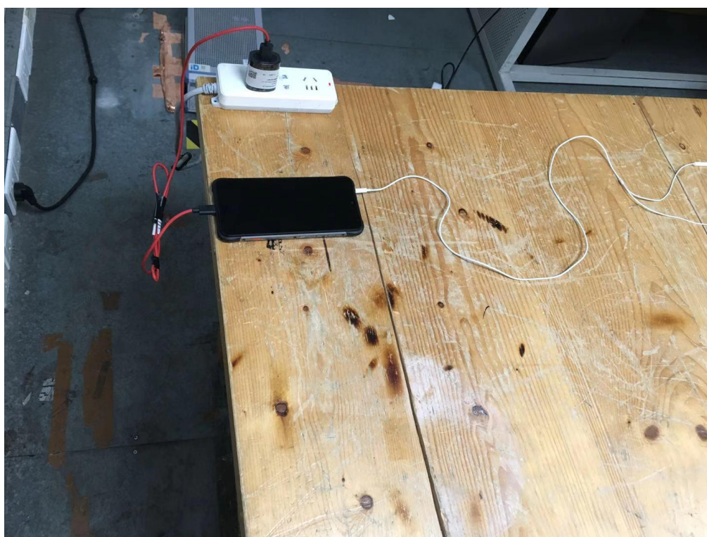
Photo of Conducted Emission Measurement – Rear
