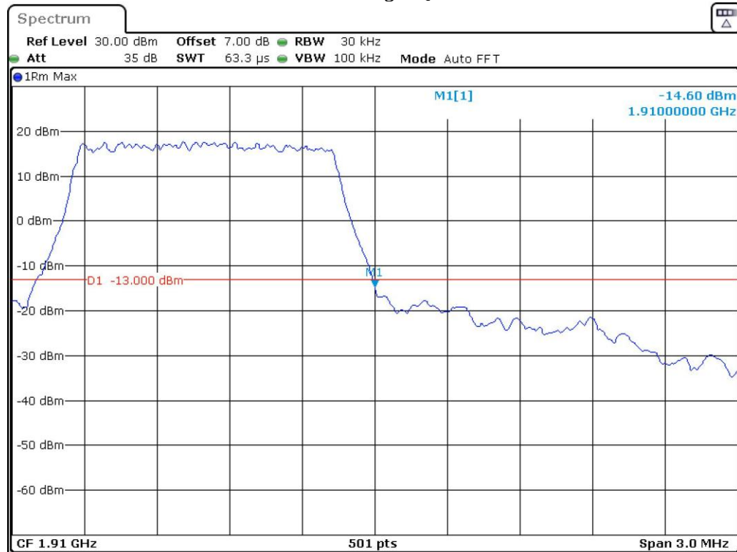
Band 2_1.4 MHz_High_QPSK_RB6#0
