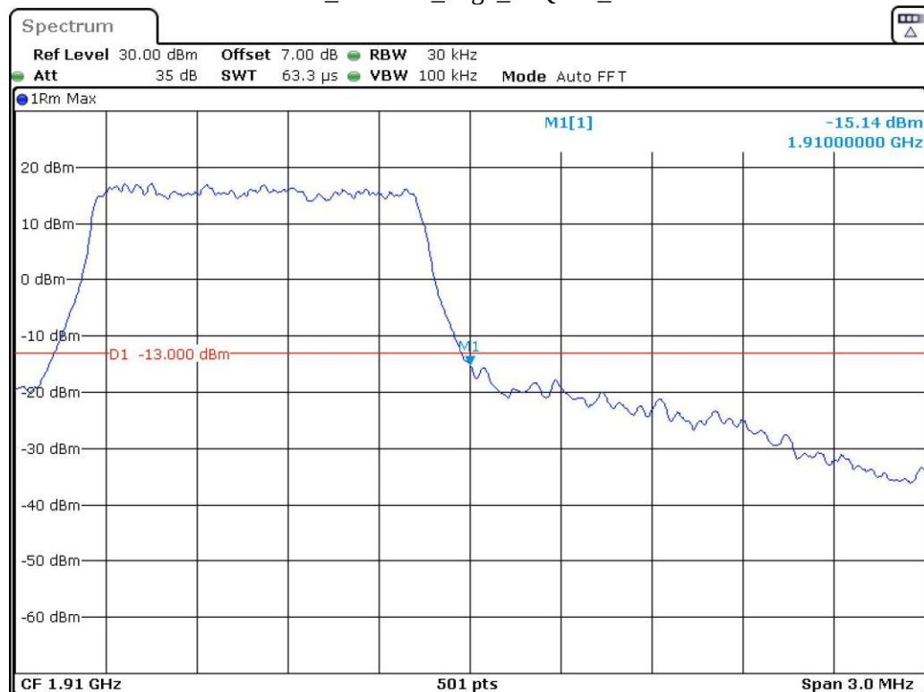
Band 2_1.4 MHz_High_16QAM_RB6#0
