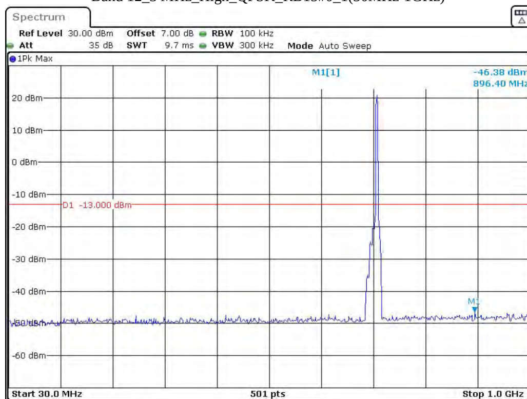
Band 12_3 MHz_High_QPSK_RB15#0_1(30MHz-1GHz)
