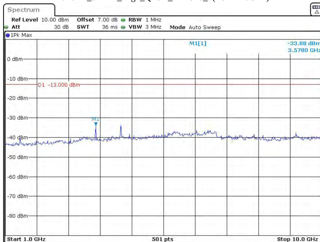
Band 12_3 MHz_High_QPSK_RB15#0_2(1GHz-10GHz)
