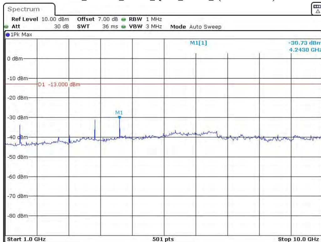
Band 12_1.4 MHz_Middle_QPSK_RB6#0_2(1GHz-10GHz)
