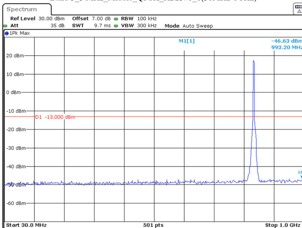
Band 5 5 MHz Middle QPSK RB25#0 1(30MHz-1GHz)
