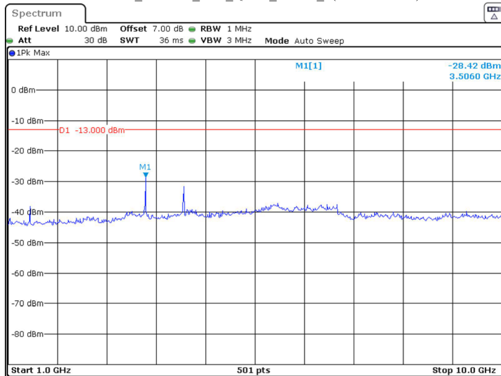
Band 12_1.4 MHz_Low_QPSK_RB6#0_2(1GHz-10GHz)
