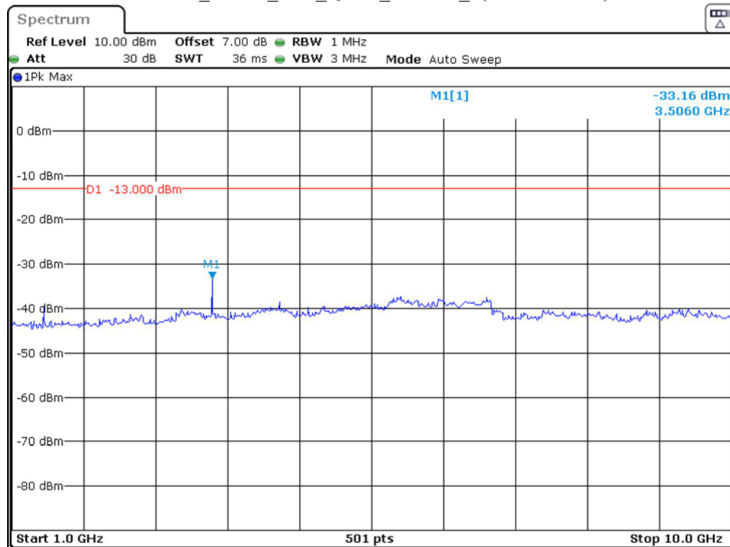
Band 12_3 MHz_Low_QPSK_RB15#0_2(1GHz-10GHz)
