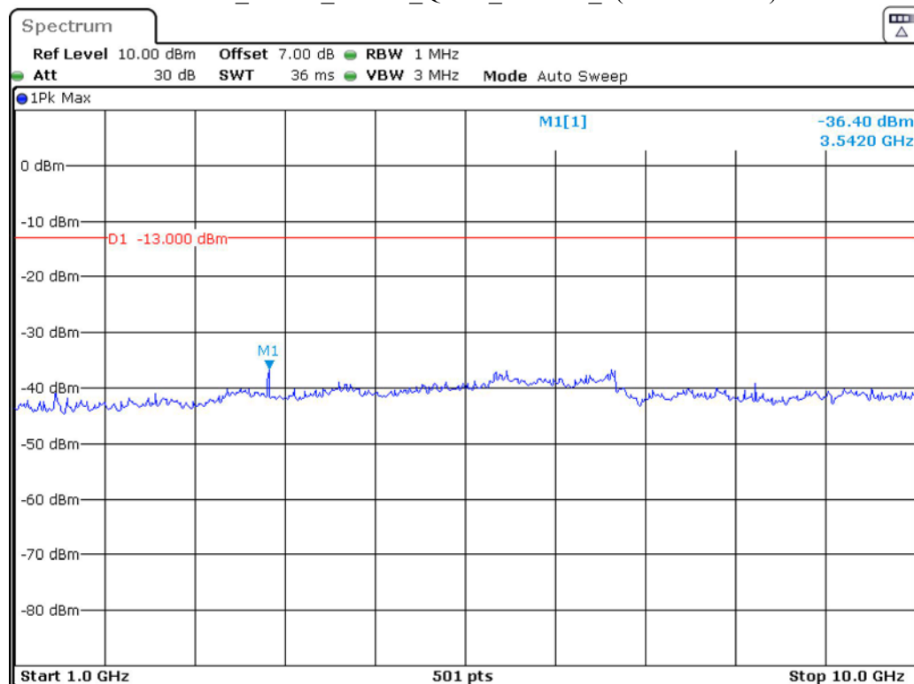
Band 12_5 MHz_Middle_QPSK_RB25#0_2(1GHz-10GHz)
