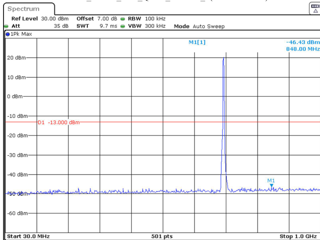
Band 12_3 MHz_Low_QPSK_RB15#0_1(30MHz-1GHz)
