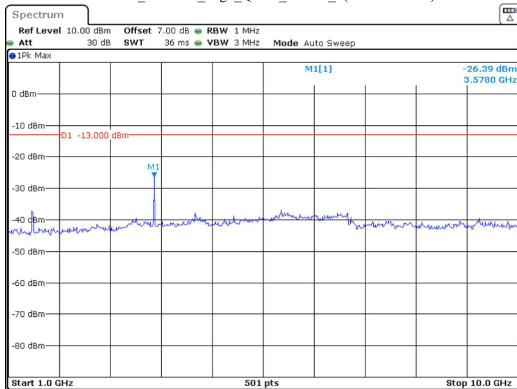
Band 12_1.4 MHz_High_QPSK_RB6#0_2(1GHz-10GHz)
