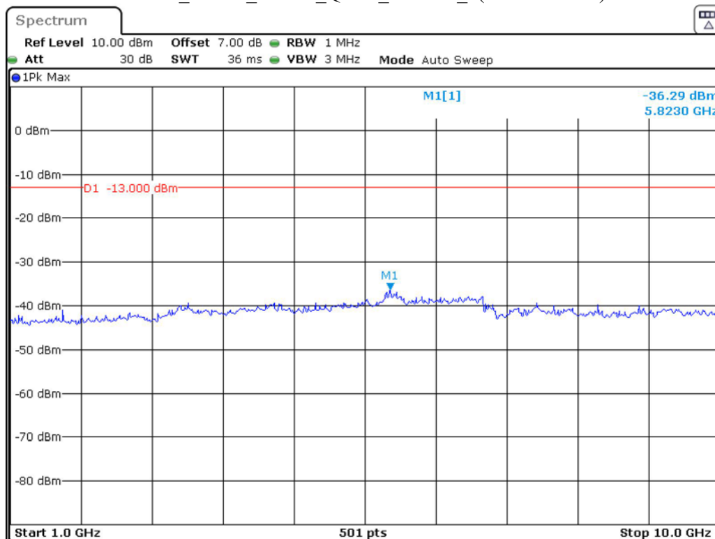
Band 5 5 MHz Middle QPSK RB25#0 2(1GHz-10GHz)
